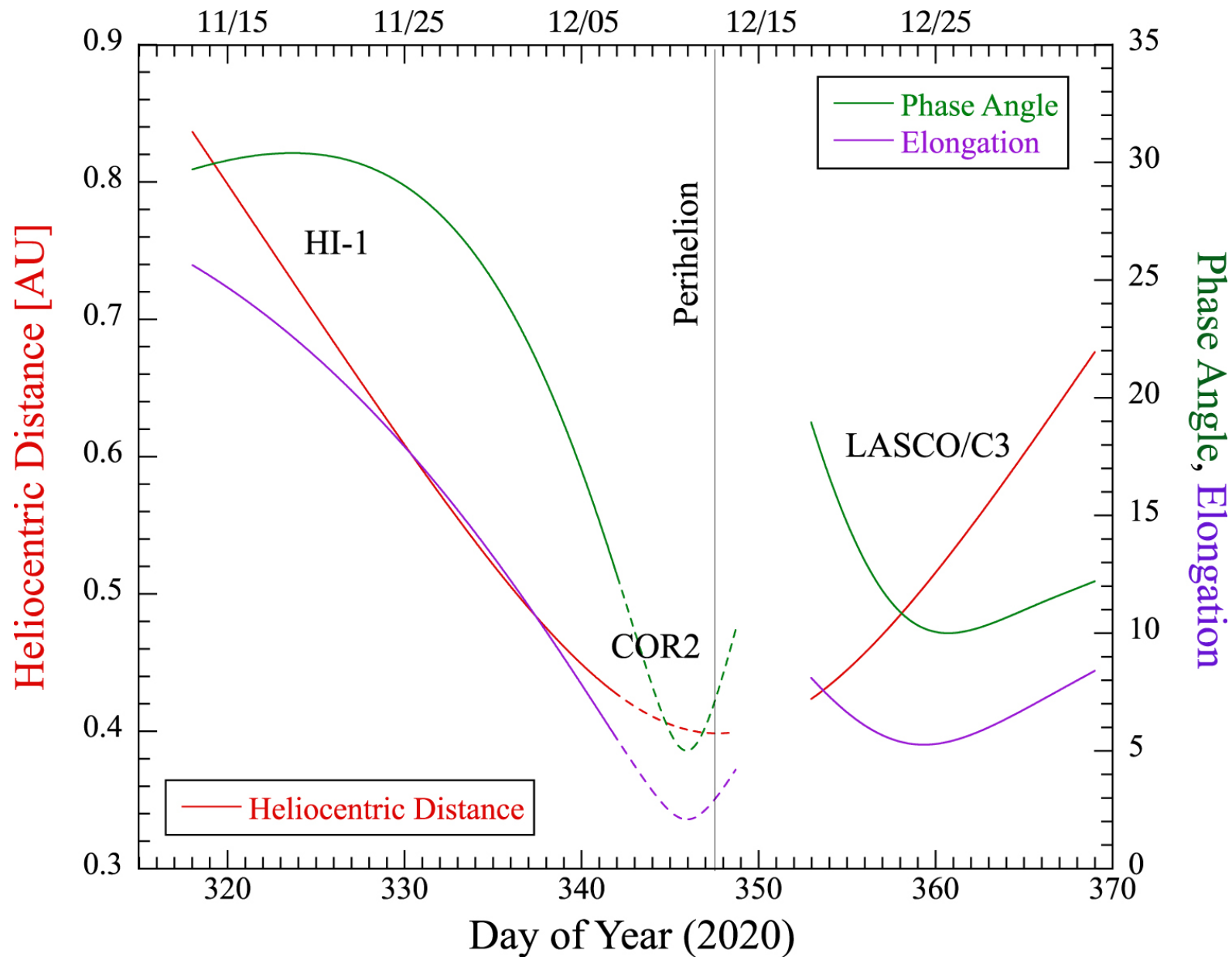
Figure 2. from Jing Li et al 2023 Astron. J. 166 doi:10.3847/1538-3881/ad08af https://dx.doi.org/10.3847/1538-3881/ad08af © 2023. The Author(s). Published by the American Astronomical Society.
