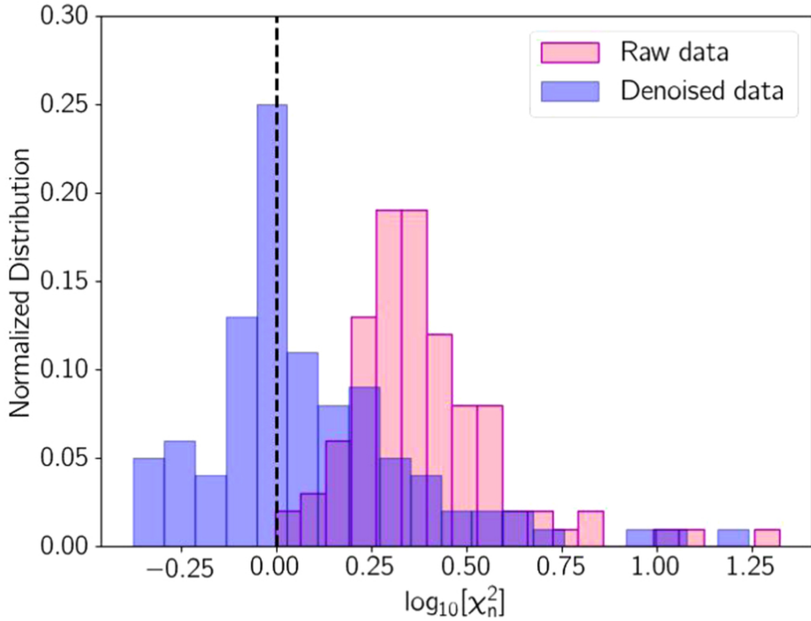
Figure 5. from Sedighe Sajadian and Hossein Fatheddin 2023 Astron. J. 166 doi:10.3847/1538-3881/ad07d9 https://dx.doi.org/10.3847/1538-3881/ad07d9 © 2023. The Author(s). Published by the American Astronomical Society.
