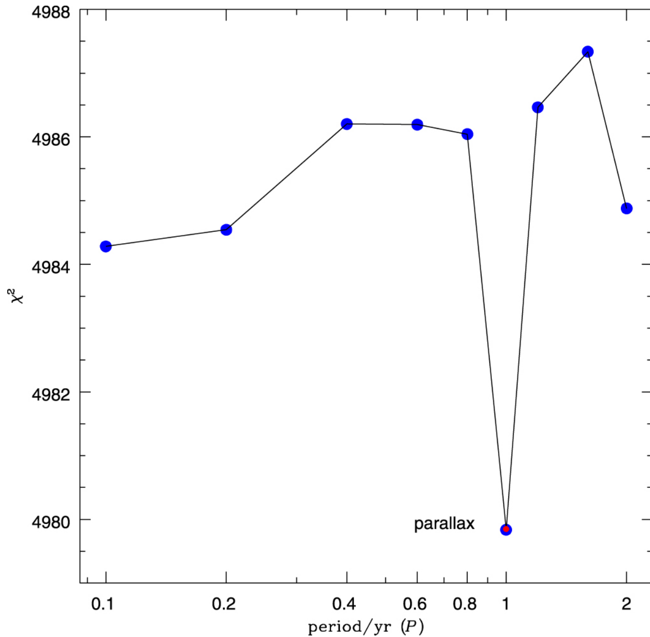
Figure 8. from Sun-Ju Chung et al 2023 Astron. J. 166 doi:10.3847/1538-3881/ad0723 https://dx.doi.org/10.3847/1538-3881/ad0723 © 2023. The Author(s). Published by the American Astronomical Society.
