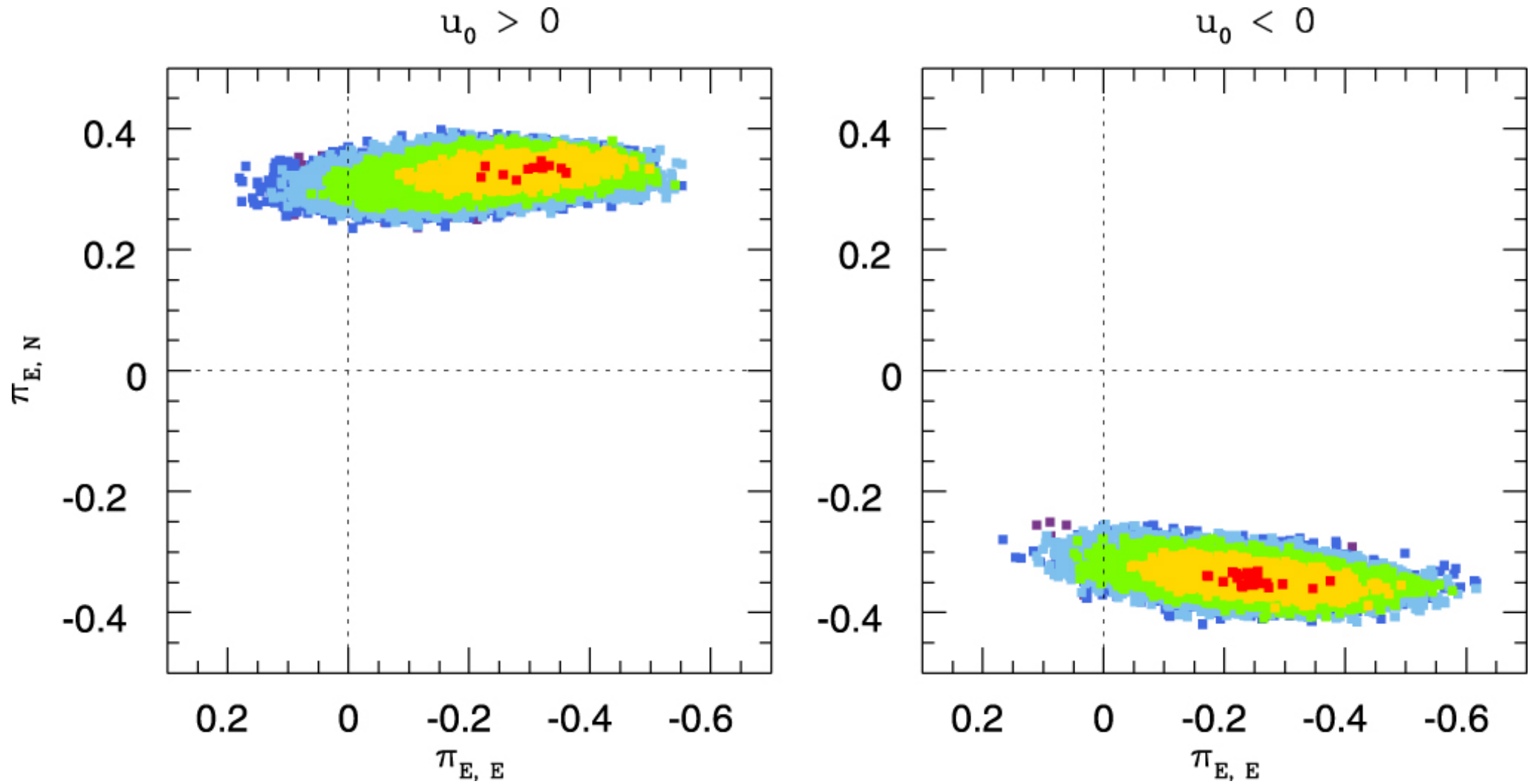
Figure 6. from Sun-Ju Chung et al 2023 Astron. J. 166 doi:10.3847/1538-3881/ad0723 https://dx.doi.org/10.3847/1538-3881/ad0723 © 2023. The Author(s). Published by the American Astronomical Society.
