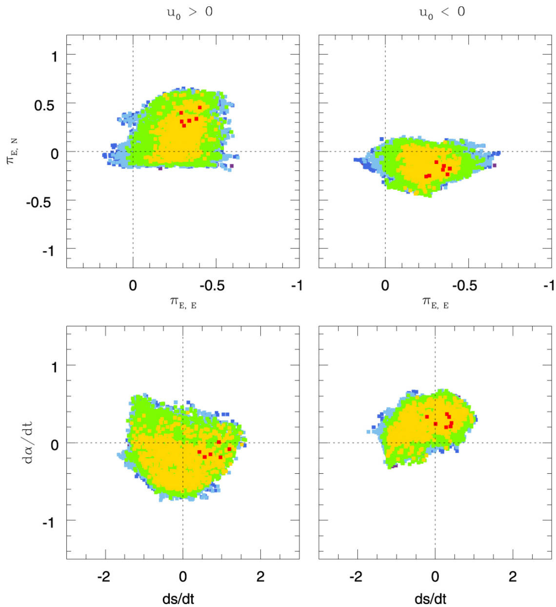
Figure 5. from Sun-Ju Chung et al 2023 Astron. J. 166 doi:10.3847/1538-3881/ad0723 https://dx.doi.org/10.3847/1538-3881/ad0723 © 2023. The Author(s). Published by the American Astronomical Society.
