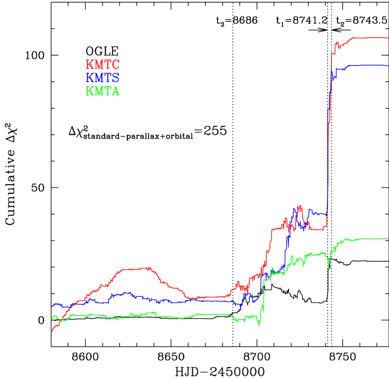
Figure 4. from Sun-Ju Chung et al 2023 Astron. J. 166 doi:10.3847/1538-3881/ad0723 https://dx.doi.org/10.3847/1538-3881/ad0723 © 2023. The Author(s). Published by the American Astronomical Society.
