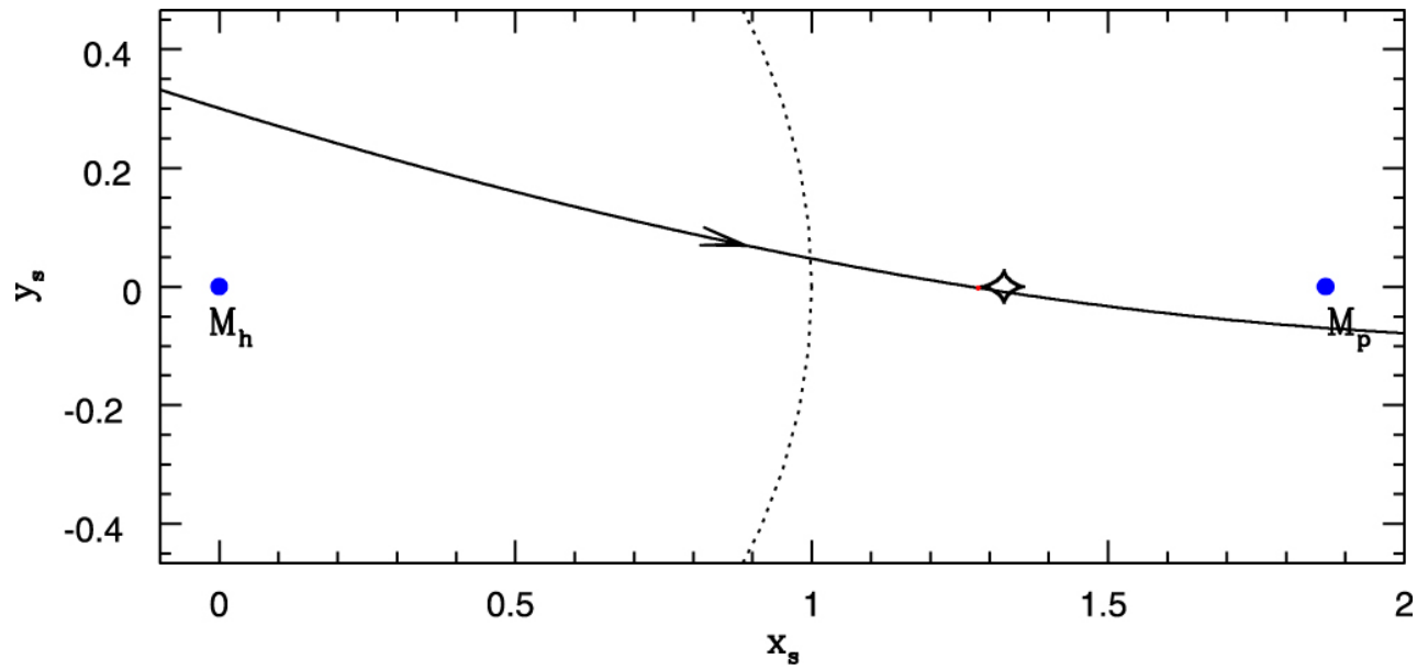
Figure 3. from Sun-Ju Chung et al 2023 Astron. J. 166 doi:10.3847/1538-3881/ad0723 https://dx.doi.org/10.3847/1538-3881/ad0723 © 2023. The Author(s). Published by the American Astronomical Society.
