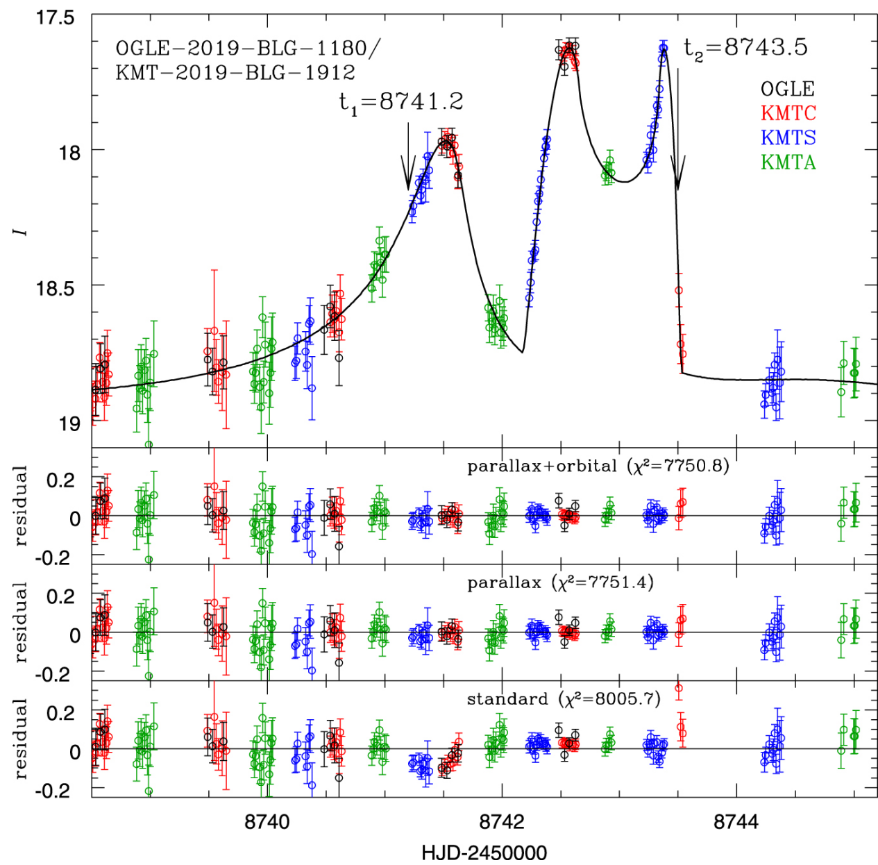
Figure 2. from Sun-Ju Chung et al 2023 Astron. J. 166 doi:10.3847/1538-3881/ad0723 https://dx.doi.org/10.3847/1538-3881/ad0723 © 2023. The Author(s). Published by the American Astronomical Society.
