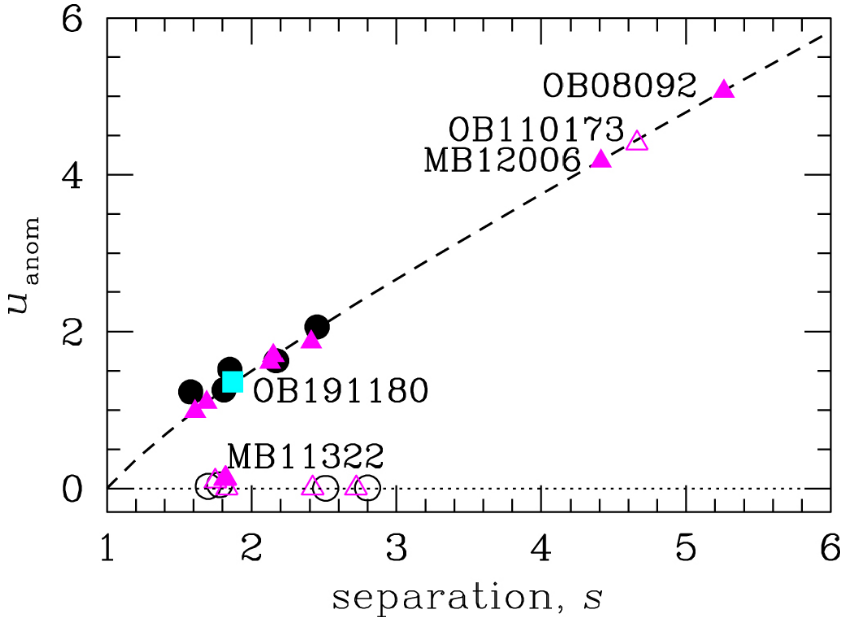
Figure 12. from Sun-Ju Chung et al 2023 Astron. J. 166 doi:10.3847/1538-3881/ad0723 https://dx.doi.org/10.3847/1538-3881/ad0723 © 2023. The Author(s). Published by the American Astronomical Society.
