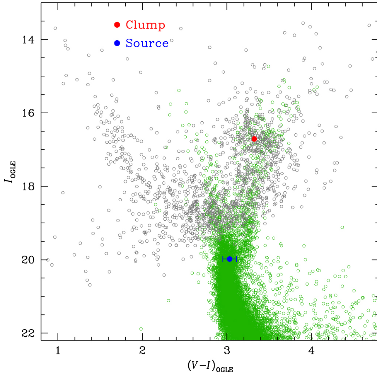
Figure 10. from Sun-Ju Chung et al 2023 Astron. J. 166 doi:10.3847/1538-3881/ad0723 https://dx.doi.org/10.3847/1538-3881/ad0723 © 2023. The Author(s). Published by the American Astronomical Society.
