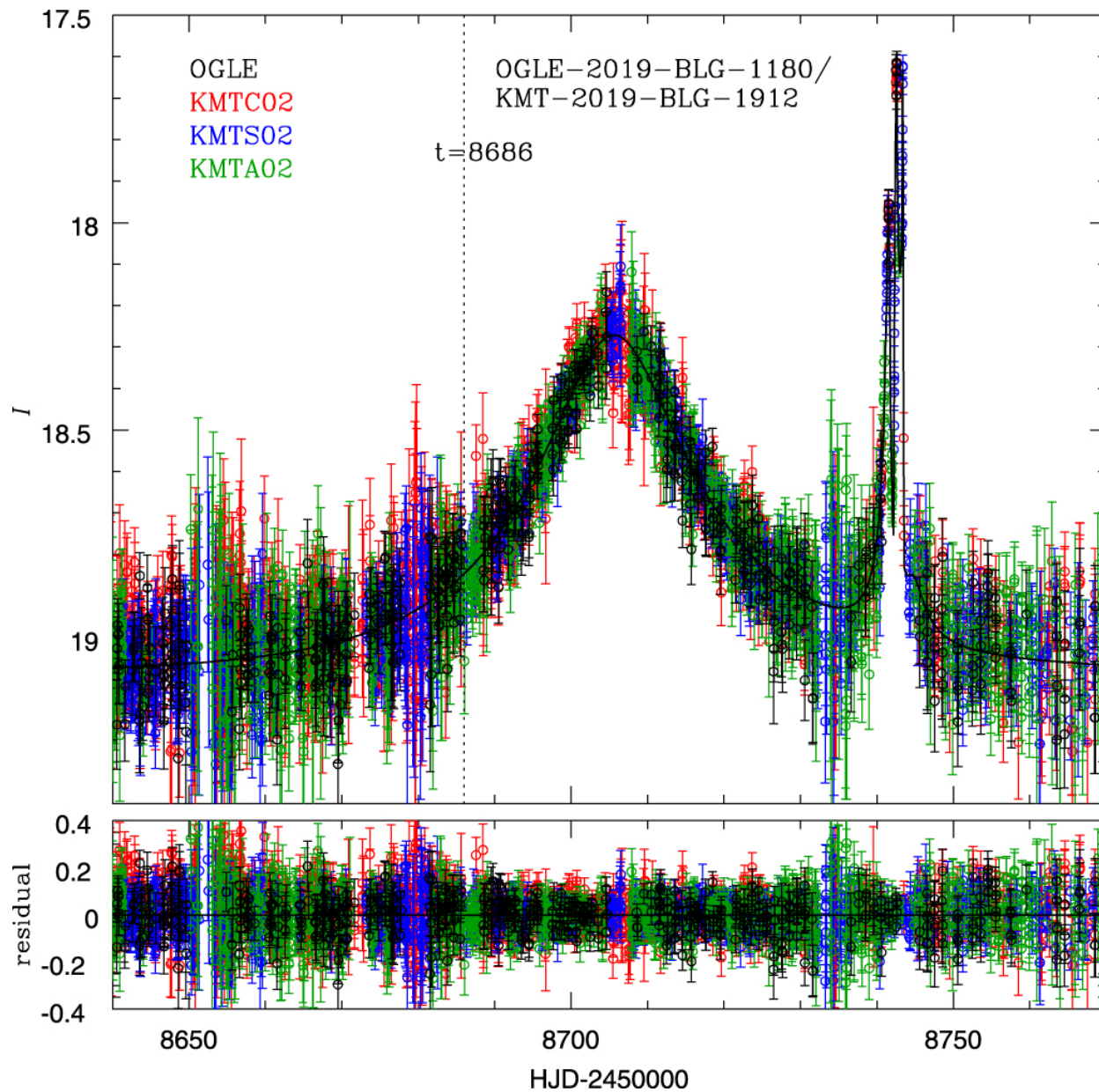
Figure 1. from Sun-Ju Chung et al 2023 Astron. J. 166 doi:10.3847/1538-3881/ad0723 https://dx.doi.org/10.3847/1538-3881/ad0723 © 2023. The Author(s). Published by the American Astronomical Society.
