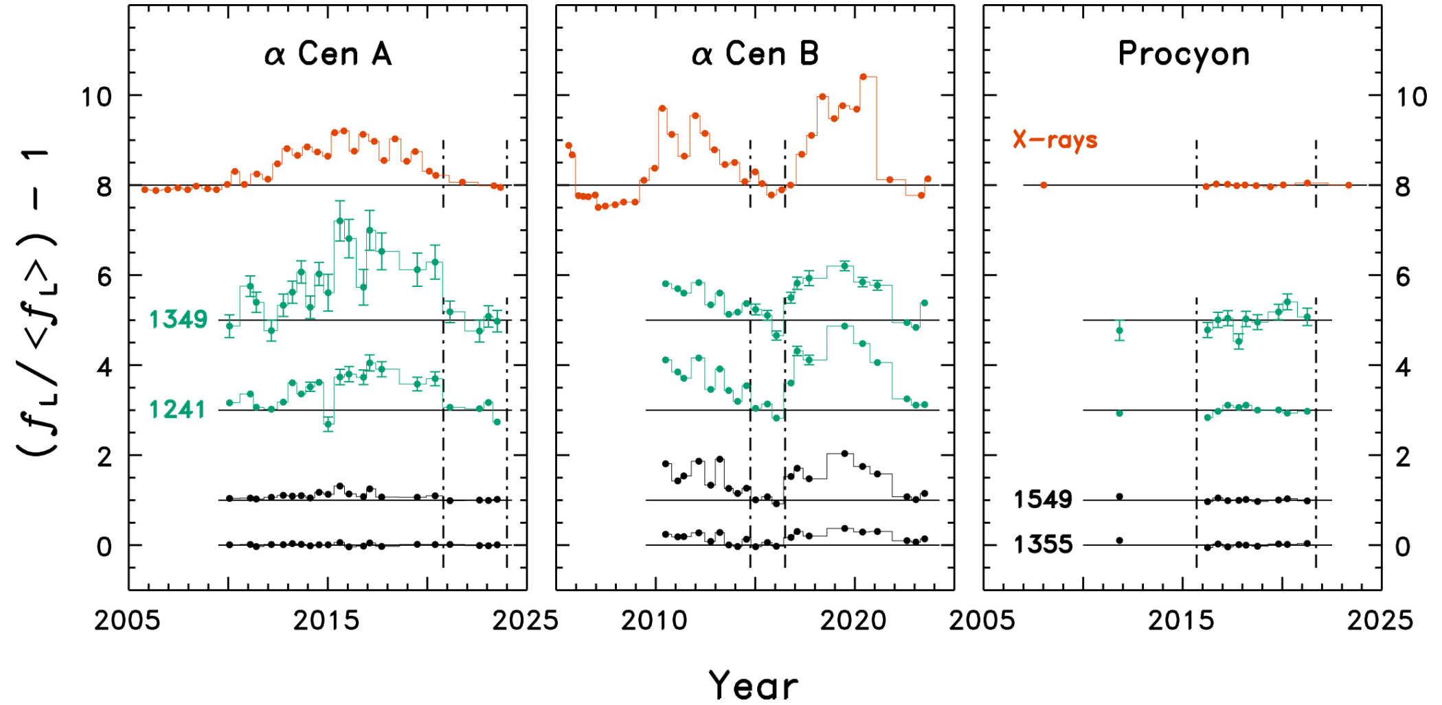
Figure 5. from Thomas Ayres 2023 Astron. J. 166 doi:10.3847/1538-3881/acfef5 https://dx.doi.org/10.3847/1538-3881/acfef5 © 2023. The Author(s). Published by the American Astronomical Society.
