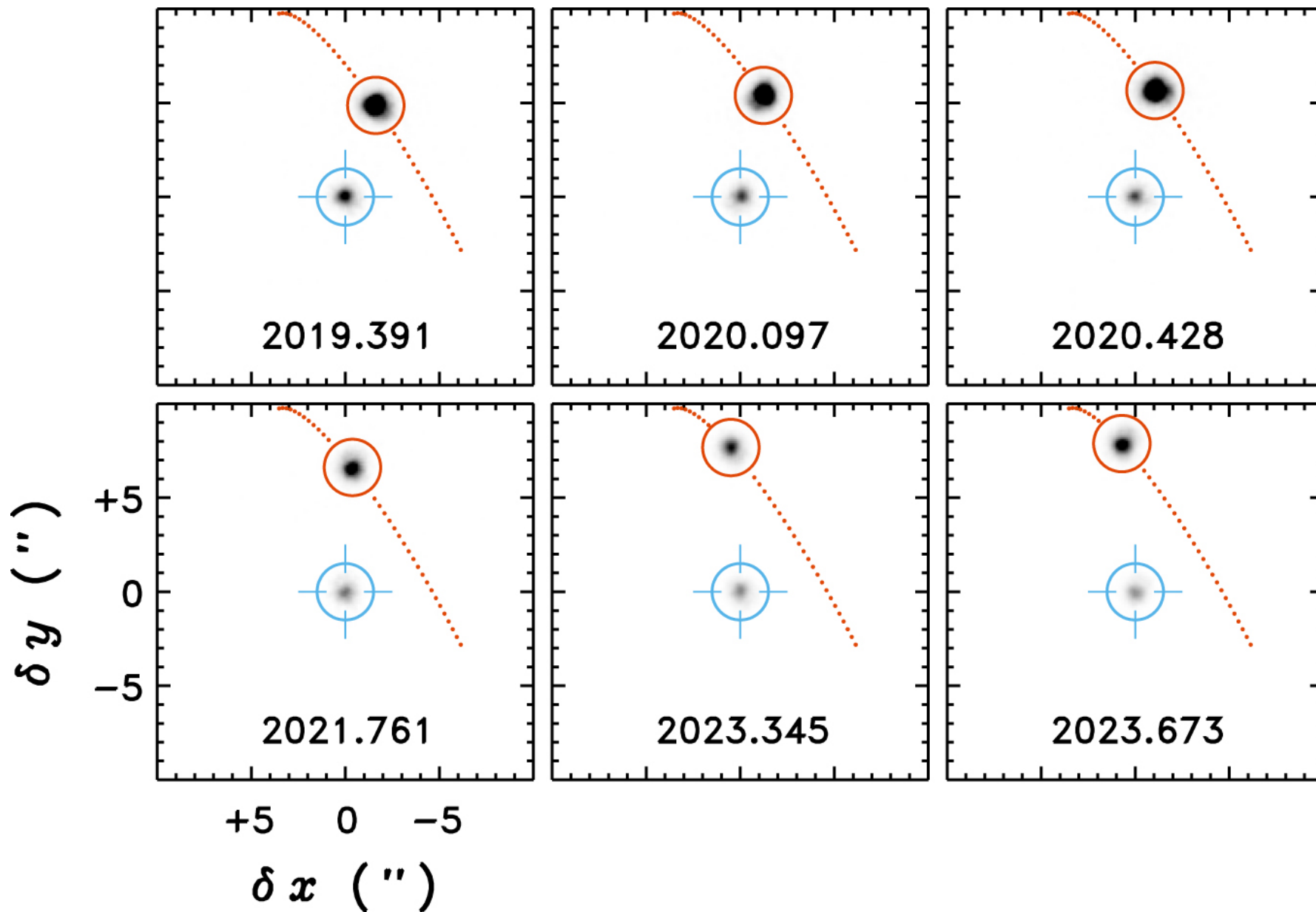
Figure 1. from Thomas Ayres 2023 Astron. J. 166 doi:10.3847/1538-3881/acfef5 https://dx.doi.org/10.3847/1538-3881/acfef5 © 2023. The Author(s). Published by the American Astronomical Society.
