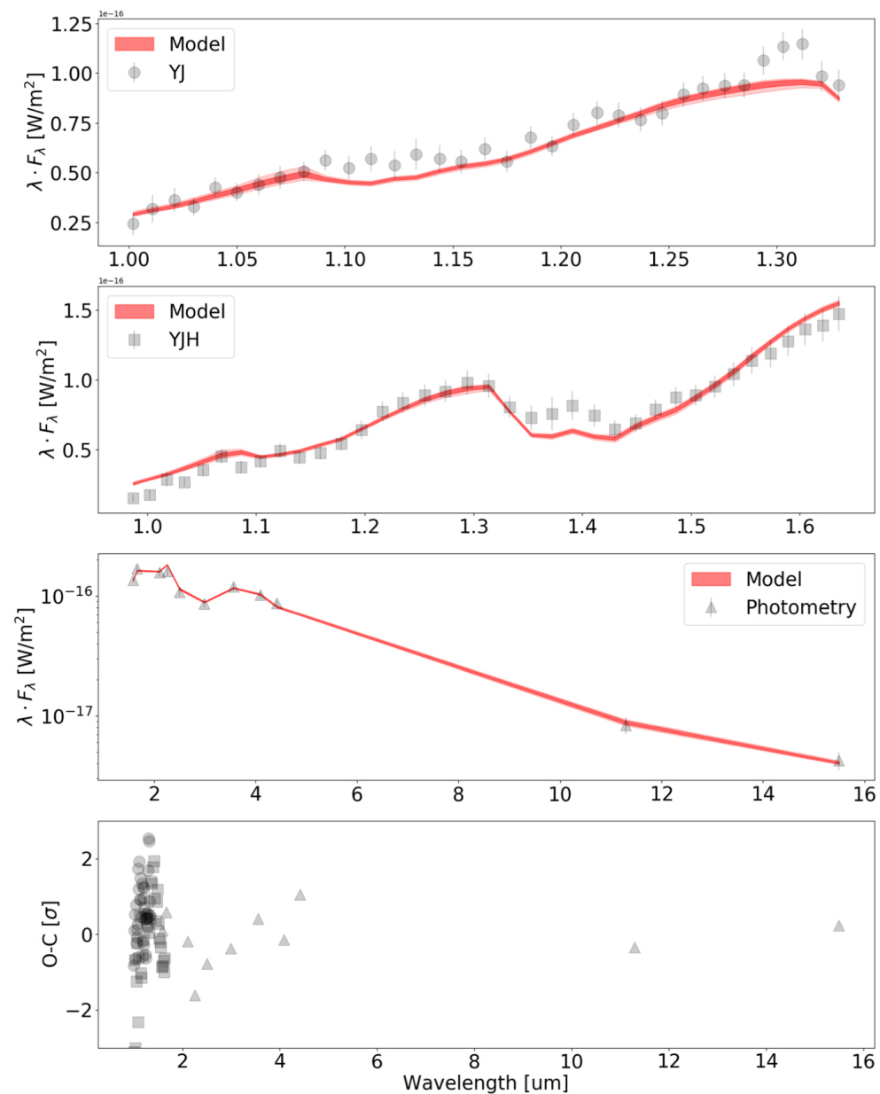
Figure 1. from Ji Wang and 2023 Astron. J. 166 doi:10.3847/1538-3881/acfca0 https://dx.doi.org/10.3847/1538-3881/acfca0 © 2023. The Author(s). Published by the American Astronomical Society.
