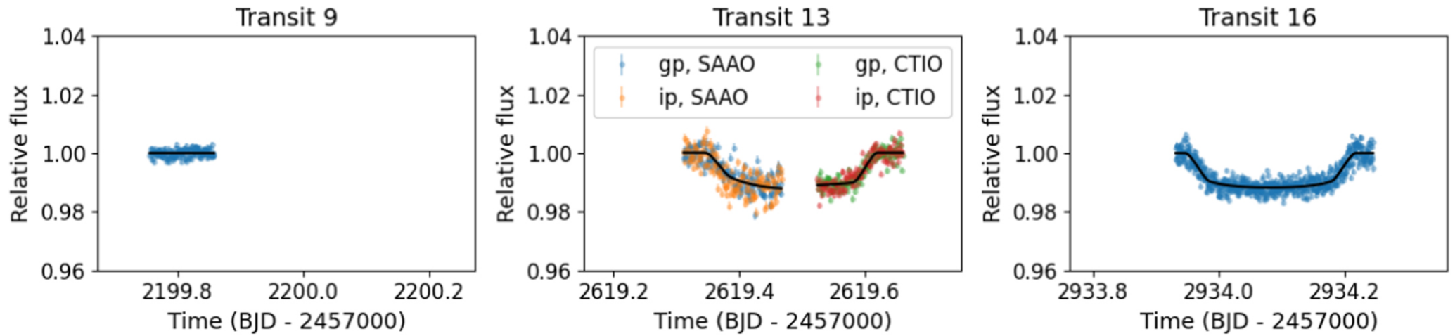
Figure 7. from Melissa J. Hobson et al 2023 Astron. J. 166 doi:10.3847/1538-3881/acfc1d https://dx.doi.org/10.3847/1538-3881/acfc1d © 2023. The Author(s). Published by the American Astronomical Society.
