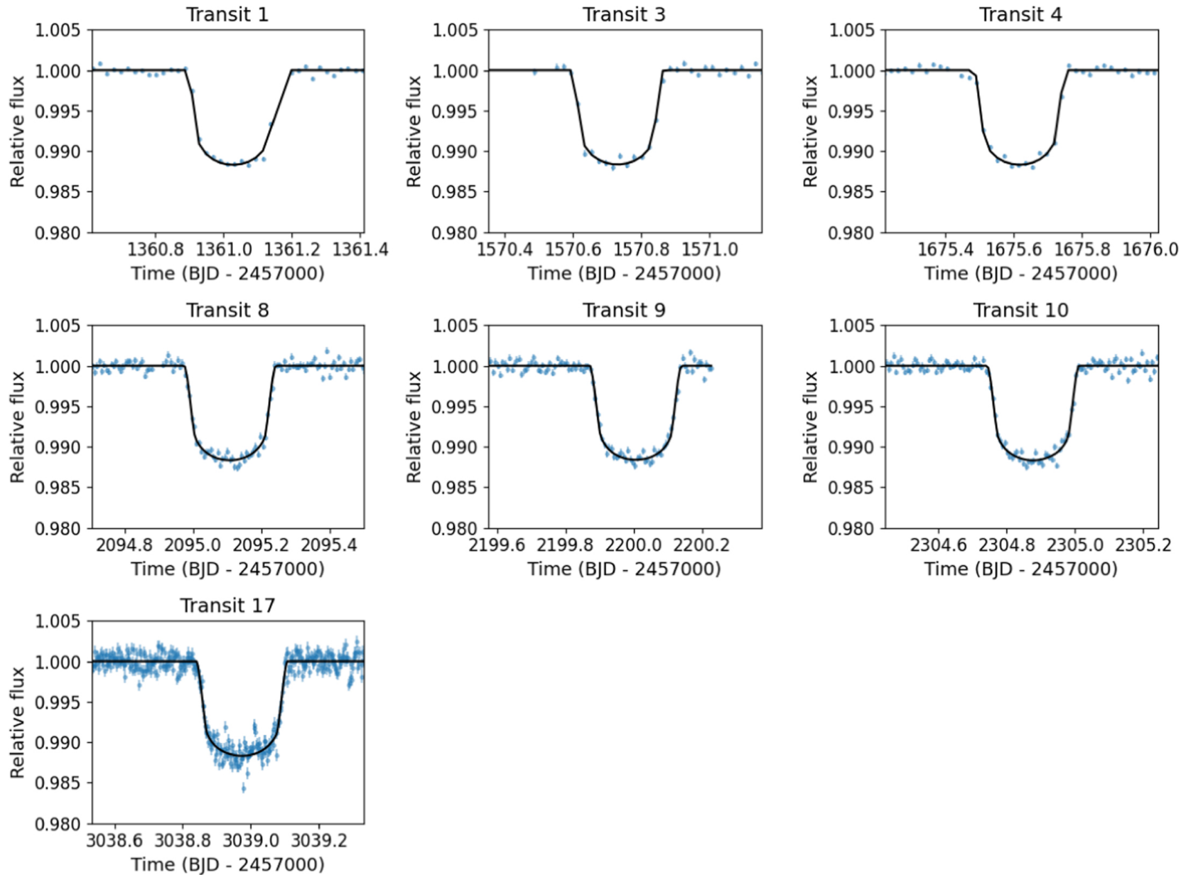
Figure 5. from Melissa J. Hobson et al 2023 Astron. J. 166 doi:10.3847/1538-3881/acfc1d https://dx.doi.org/10.3847/1538-3881/acfc1d © 2023. The Author(s). Published by the American Astronomical Society.
