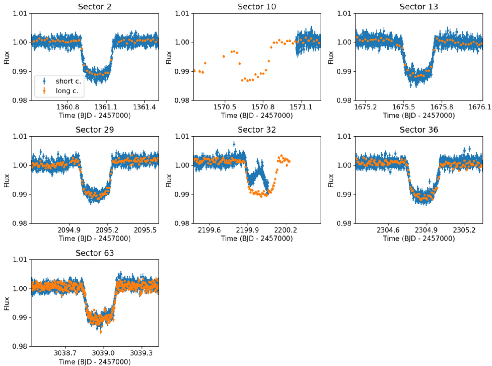
Figure 1. from Melissa J. Hobson et al 2023 Astron. J. 166 doi:10.3847/1538-3881/acfc1d https://dx.doi.org/10.3847/1538-3881/acfc1d © 2023. The Author(s). Published by the American Astronomical Society.
