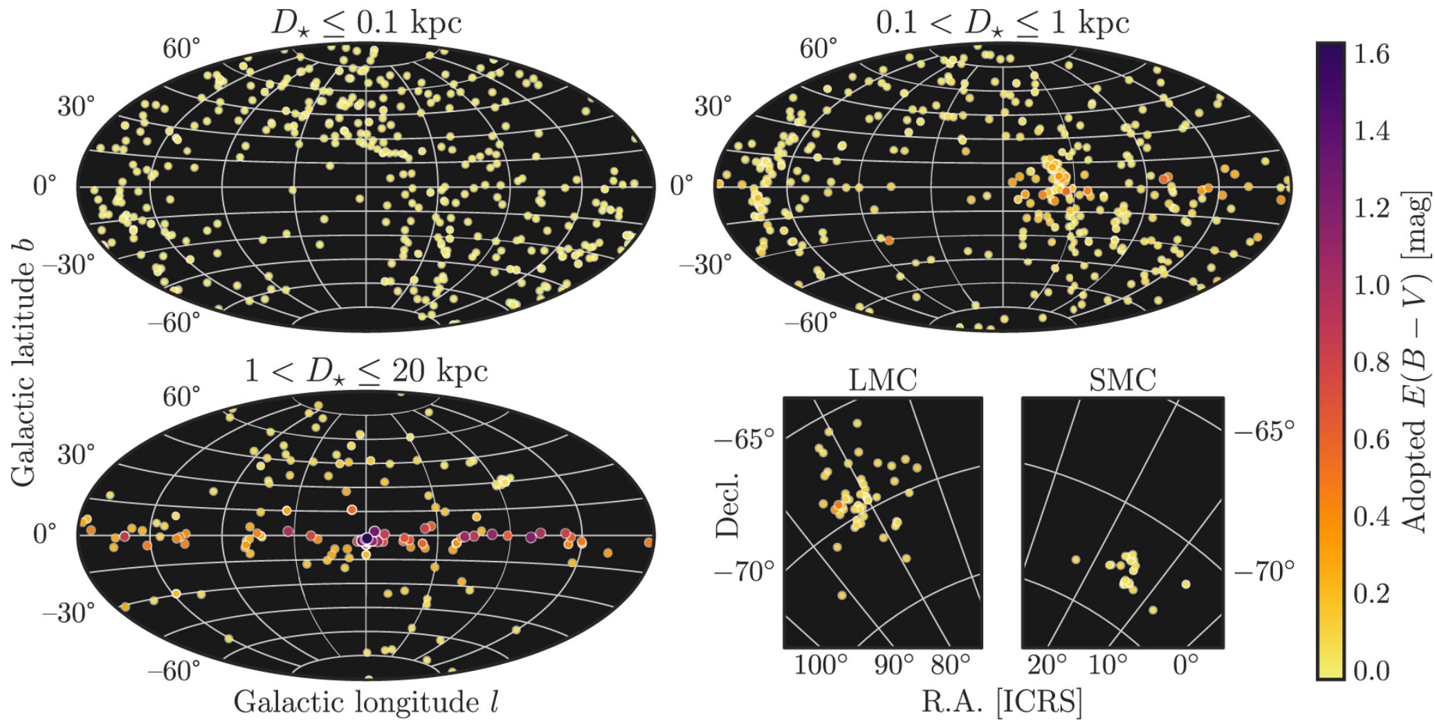
Figure 3. from M. J. Durbin et al 2023 Astron. J. 166 doi:10.3847/1538-3881/acfaa1 https://dx.doi.org/10.3847/1538-3881/acfaa1 © 2023. The Author(s). Published by the American Astronomical Society.
