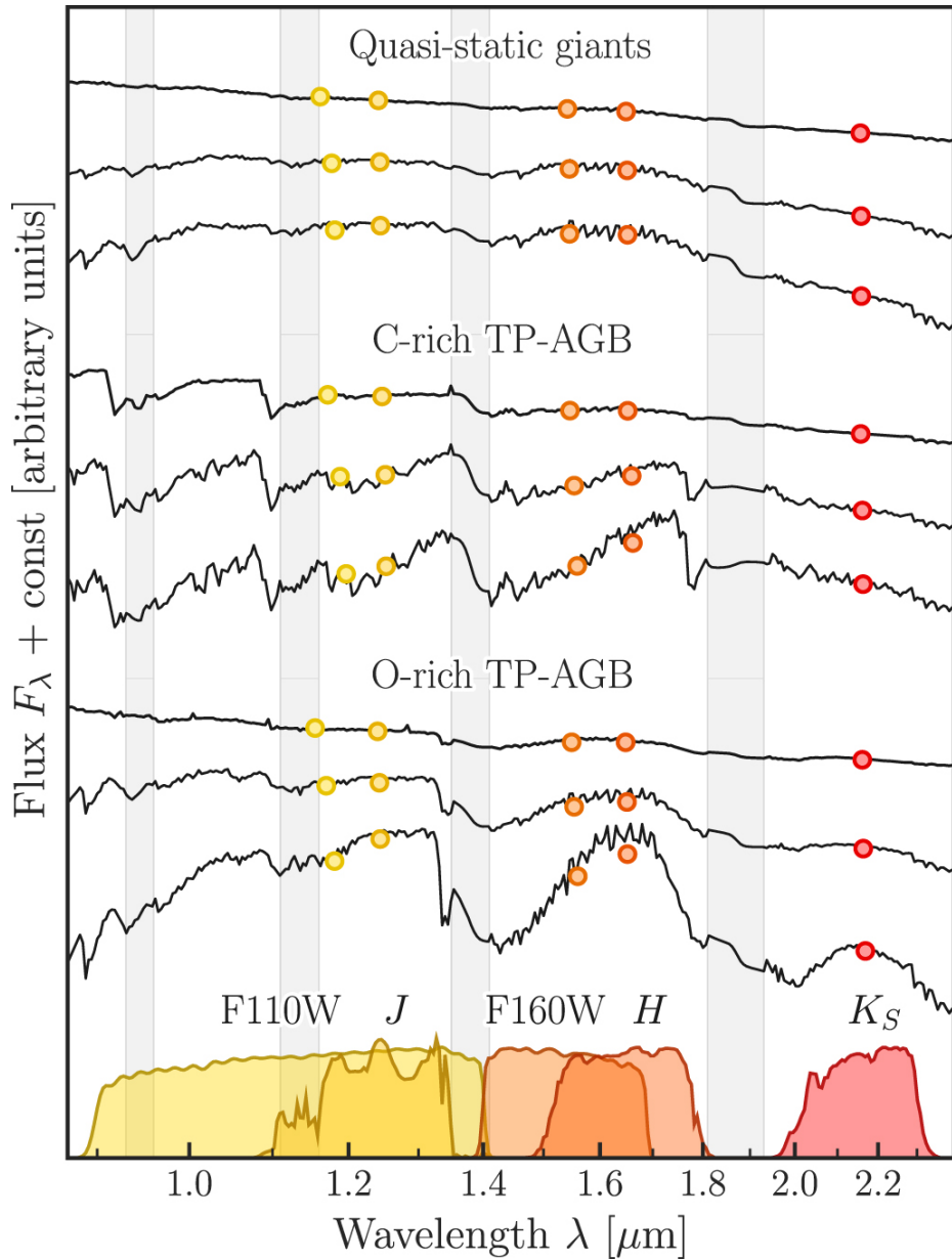
Figure 1. from M. J. Durbin et al 2023 Astron. J. 166 doi:10.3847/1538-3881/acfaa1 https://dx.doi.org/10.3847/1538-3881/acfaa1 © 2023. The Author(s). Published by the American Astronomical Society.
