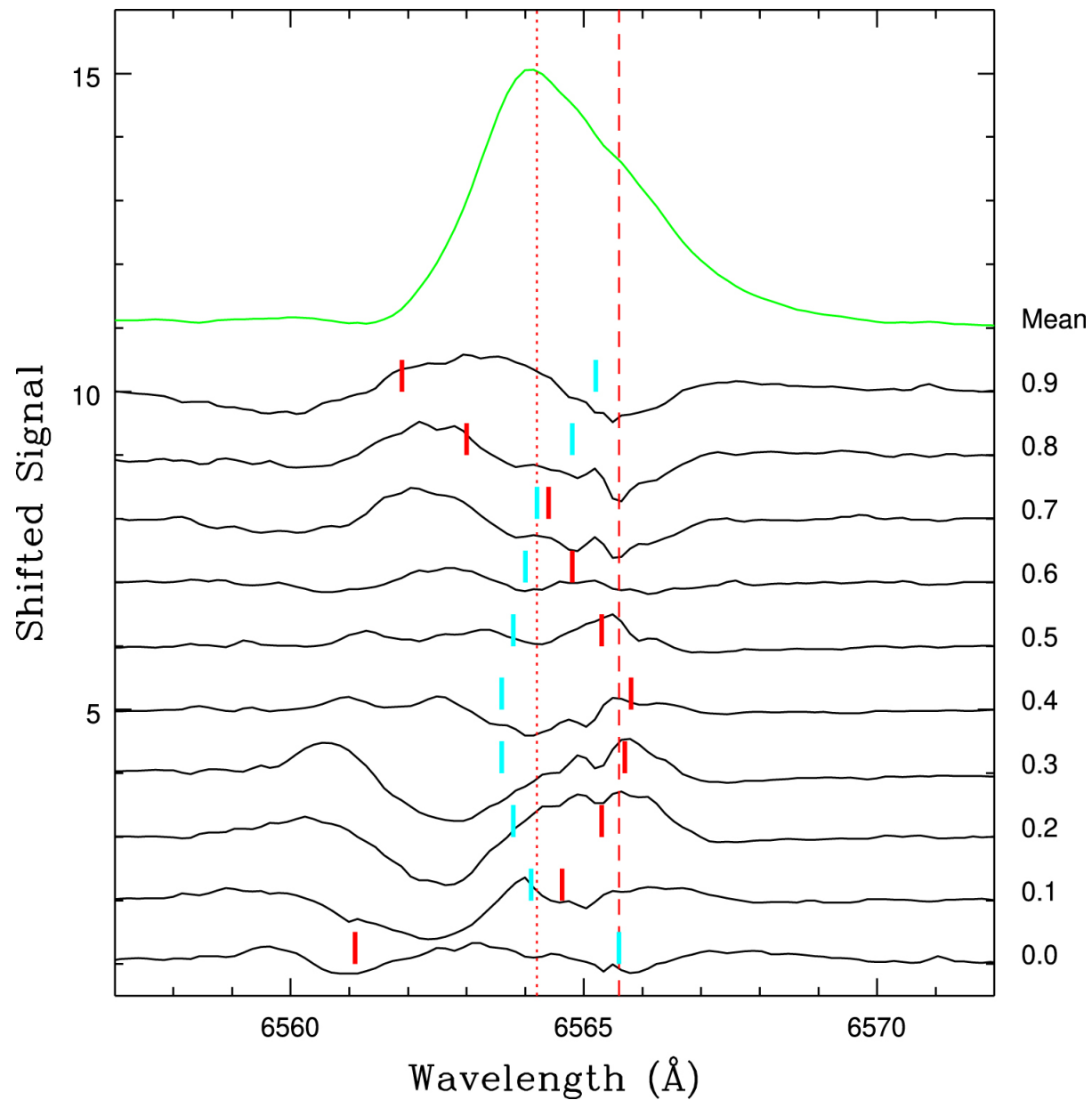
Figure 9. from T. J. Davidge 2023 Astron. J. 166 doi:10.3847/1538-3881/acfa6d https://dx.doi.org/10.3847/1538-3881/acfa6d © 2023. The Author(s). Published by the American Astronomical Society.
