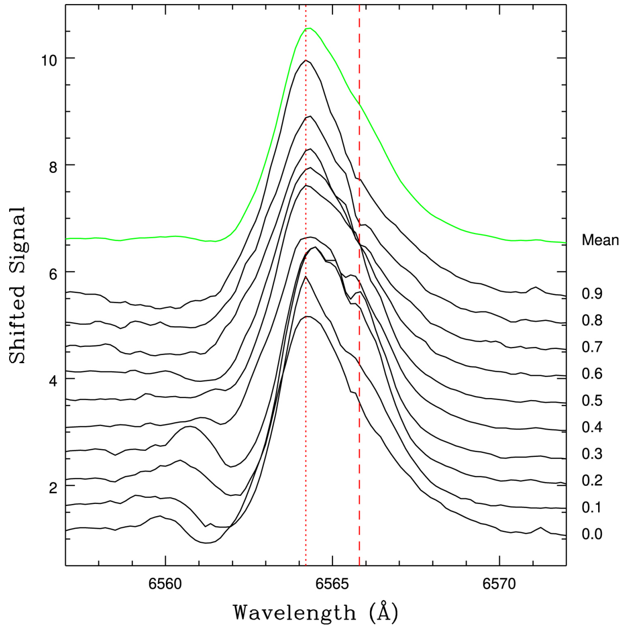
Figure 8. from T. J. Davidge 2023 Astron. J. 166 doi:10.3847/1538-3881/acfa6d https://dx.doi.org/10.3847/1538-3881/acfa6d © 2023. The Author(s). Published by the American Astronomical Society.
