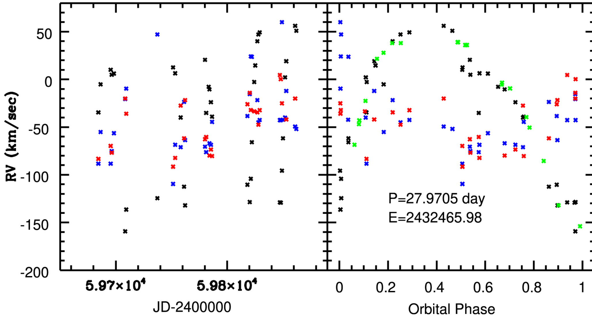
Figure 6. from T. J. Davidge 2023 Astron. J. 166 doi:10.3847/1538-3881/acfa6d https://dx.doi.org/10.3847/1538-3881/acfa6d © 2023. The Author(s). Published by the American Astronomical Society.
