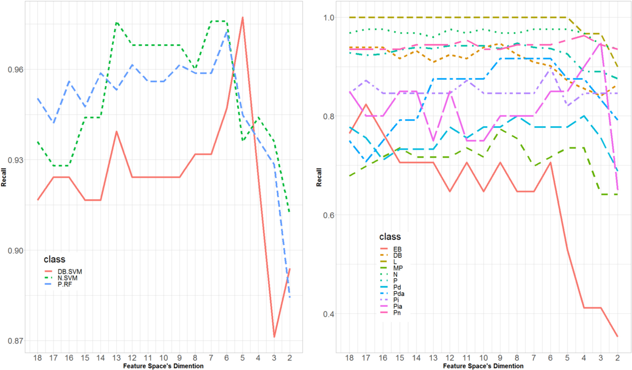
Figure 4. from Astaroth Elizabethson et al 2023 Astron. J. 166 doi:10.3847/1538-3881/acf865 https://dx.doi.org/10.3847/1538-3881/acf865 © 2023. The Author(s). Published by the American Astronomical Society.
