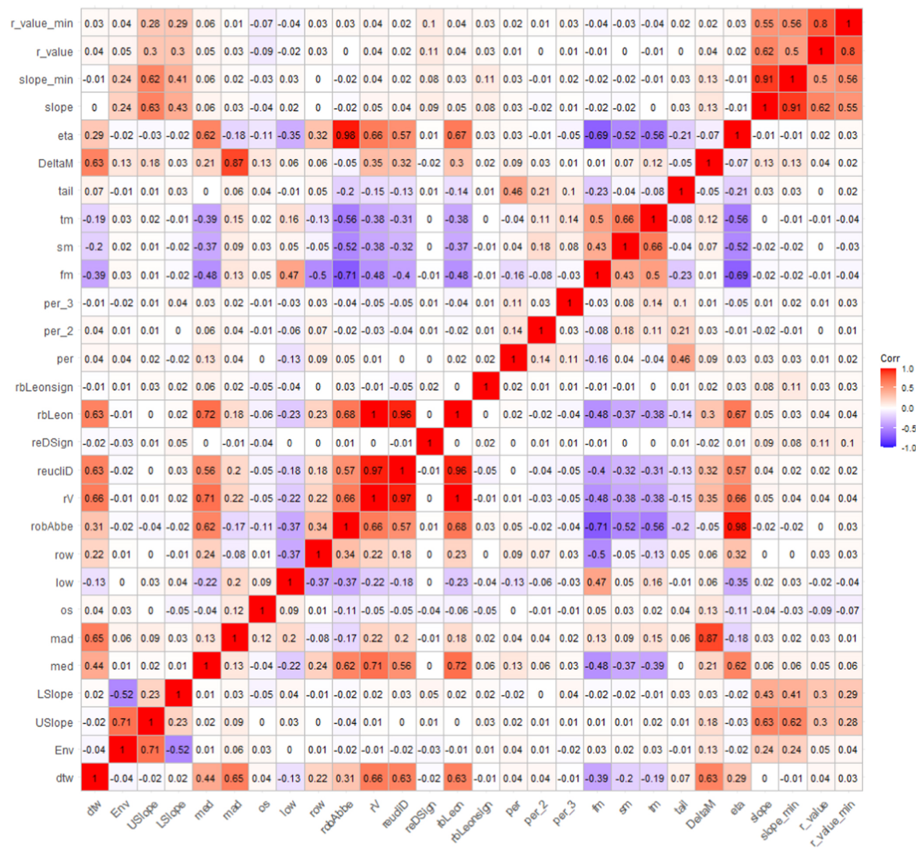
Figure 3. from Astaroth Elizabethson et al 2023 Astron. J. 166 doi:10.3847/1538-3881/acf865 https://dx.doi.org/10.3847/1538-3881/acf865 © 2023. The Author(s). Published by the American Astronomical Society.
