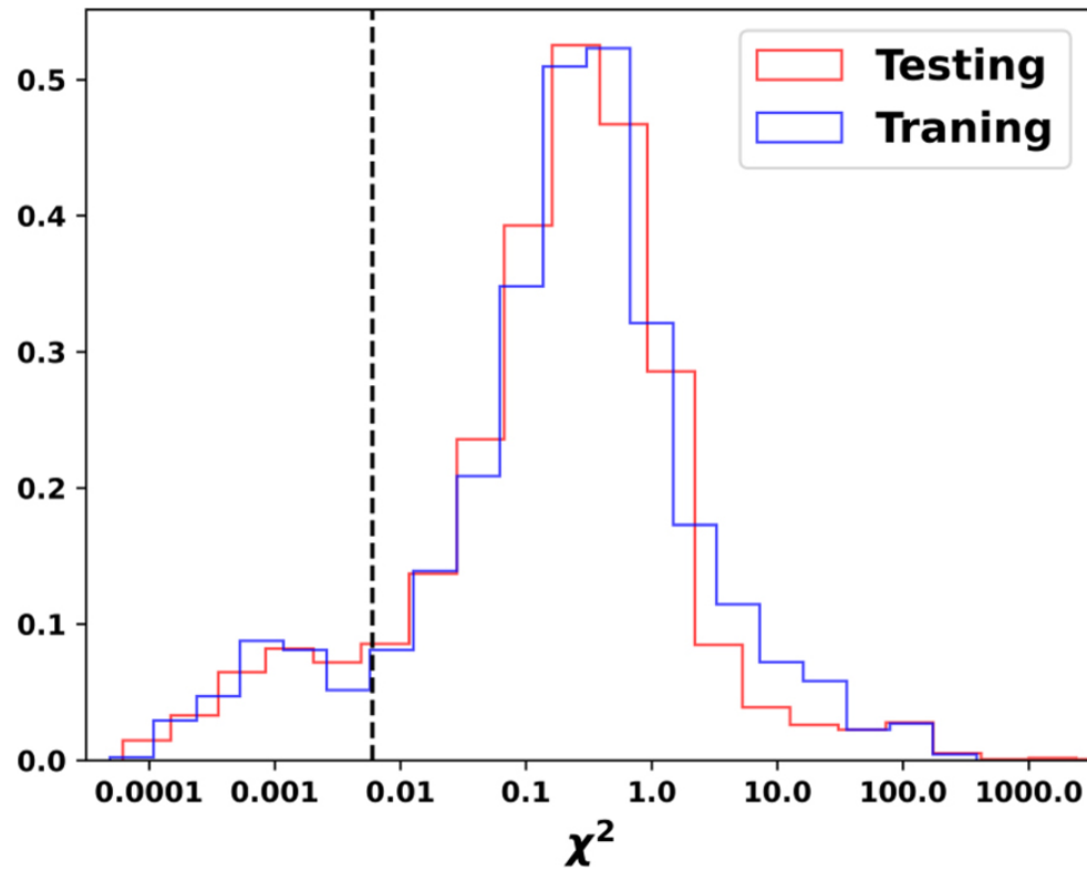
Figure 1. from Astaroth Elizabethson et al 2023 Astron. J. 166 doi:10.3847/1538-3881/acf865 https://dx.doi.org/10.3847/1538-3881/acf865 © 2023. The Author(s). Published by the American Astronomical Society.
