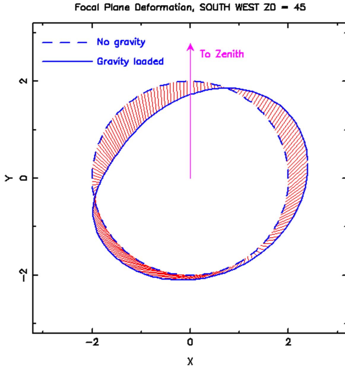
Figure 8. from S. Kent et al 2023 Astron. J. 166 doi:10.3847/1538-3881/acf7c3 https://dx.doi.org/10.3847/1538-3881/acf7c3 © 2023. The Author(s). Published by the American Astronomical Society.
