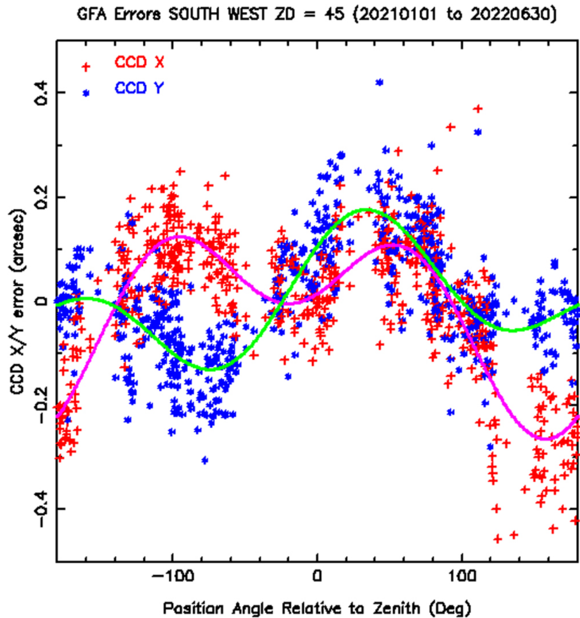
Figure 7. from S. Kent et al 2023 Astron. J. 166 doi:10.3847/1538-3881/acf7c3 https://dx.doi.org/10.3847/1538-3881/acf7c3 © 2023. The Author(s). Published by the American Astronomical Society.
