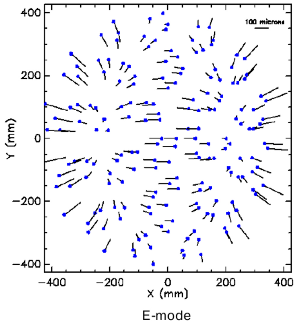
Figure 4. from S. Kent et al 2023 Astron. J. 166 doi:10.3847/1538-3881/acf7c3 https://dx.doi.org/10.3847/1538-3881/acf7c3 © 2023. The Author(s). Published by the American Astronomical Society.
