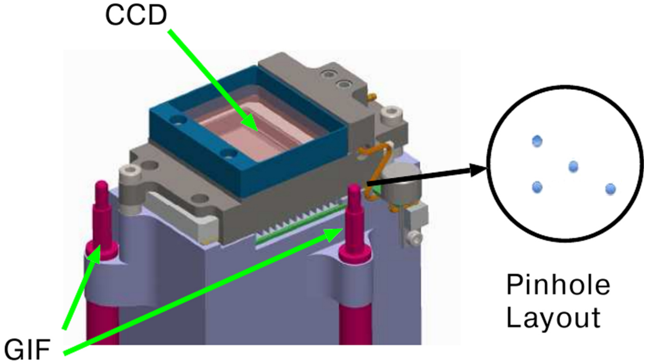
Figure 3. from S. Kent et al 2023 Astron. J. 166 doi:10.3847/1538-3881/acf7c3 https://dx.doi.org/10.3847/1538-3881/acf7c3 © 2023. The Author(s). Published by the American Astronomical Society.
