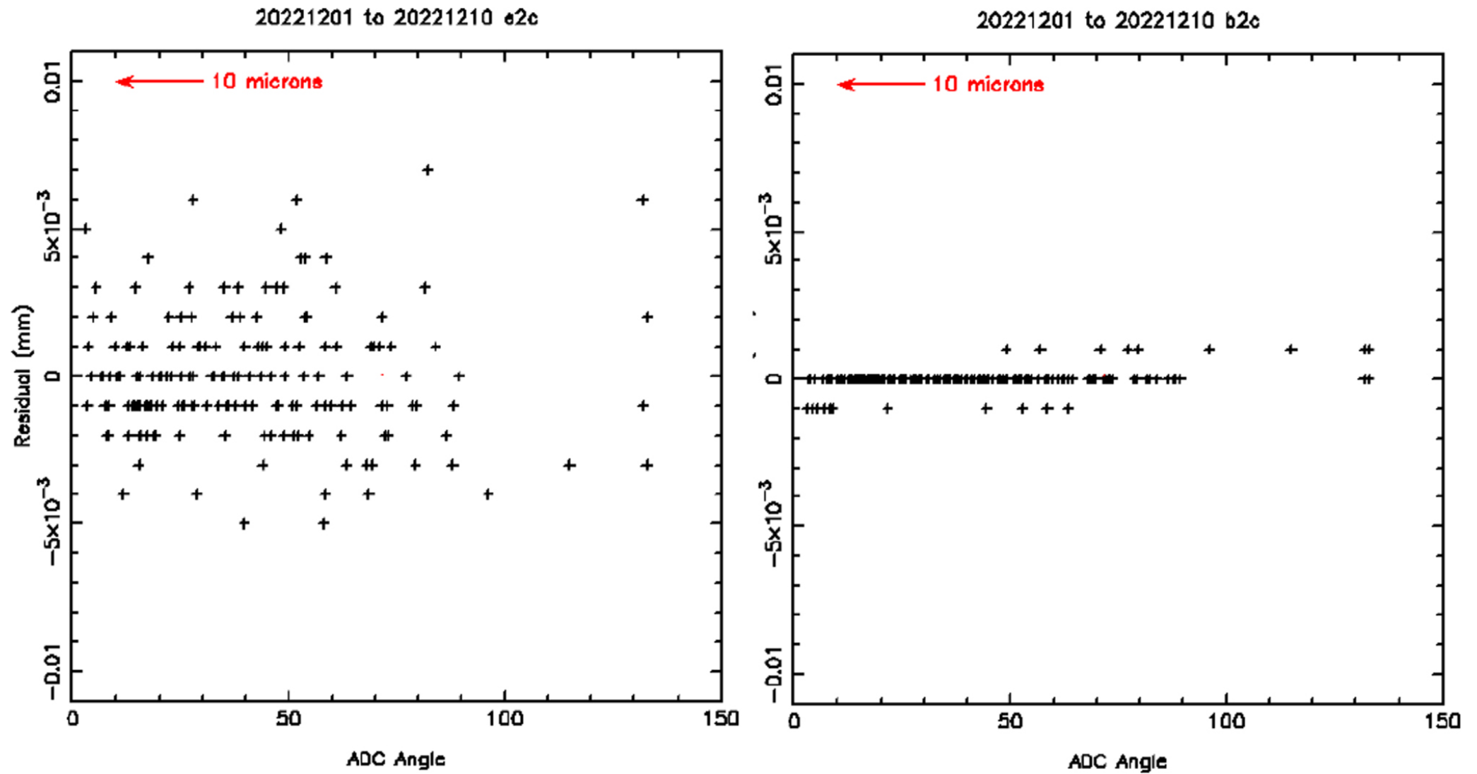
Figure 10. from S. Kent et al 2023 Astron. J. 166 doi:10.3847/1538-3881/acf7c3 https://dx.doi.org/10.3847/1538-3881/acf7c3 © 2023. The Author(s). Published by the American Astronomical Society.
