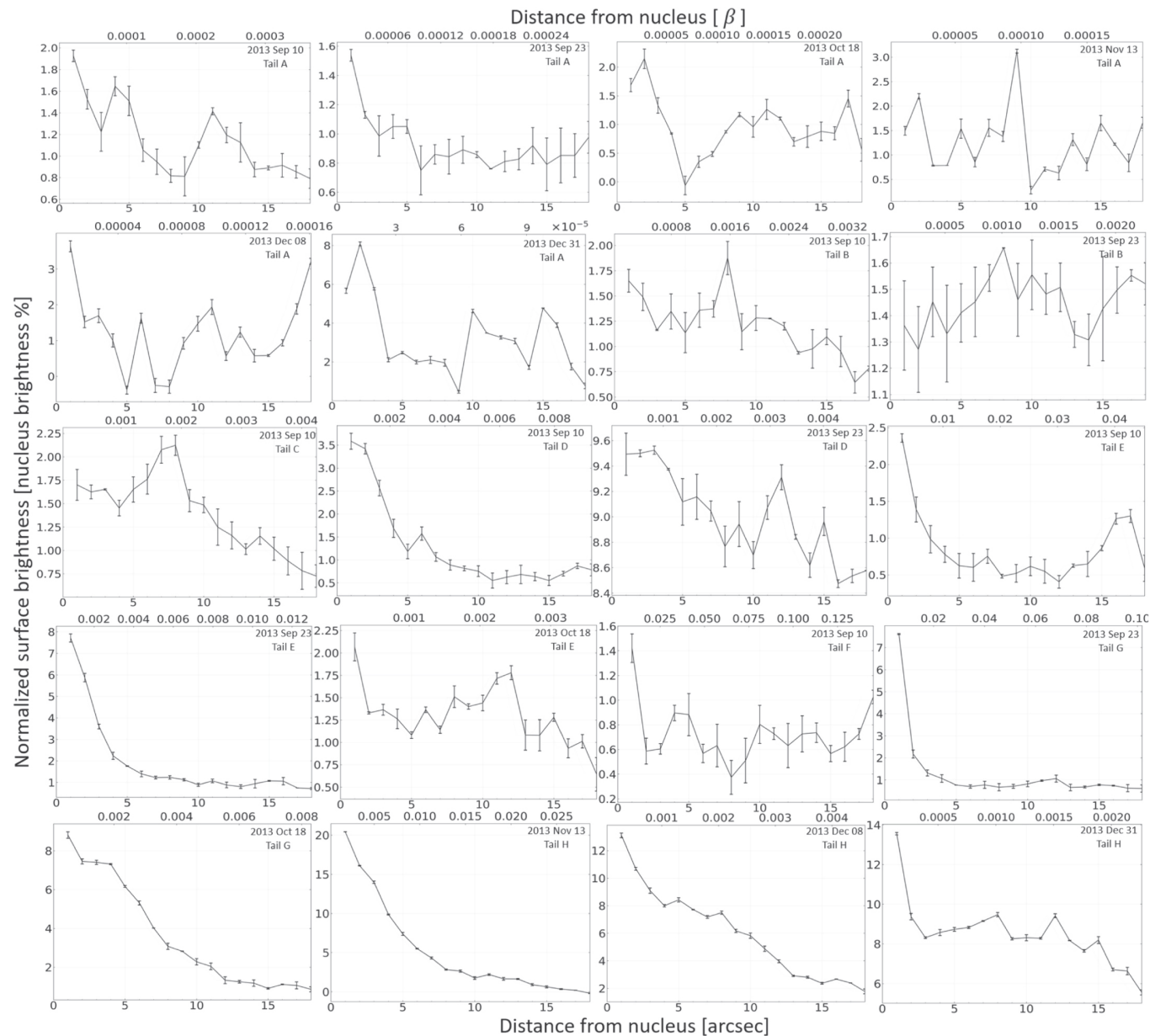
Figure 4. from Bin Liu et al 2023 Astron. J. 166 doi:10.3847/1538-3881/acf31c https://dx.doi.org/10.3847/1538-3881/acf31c © 2023. The Author(s). Published by the American Astronomical Society.
