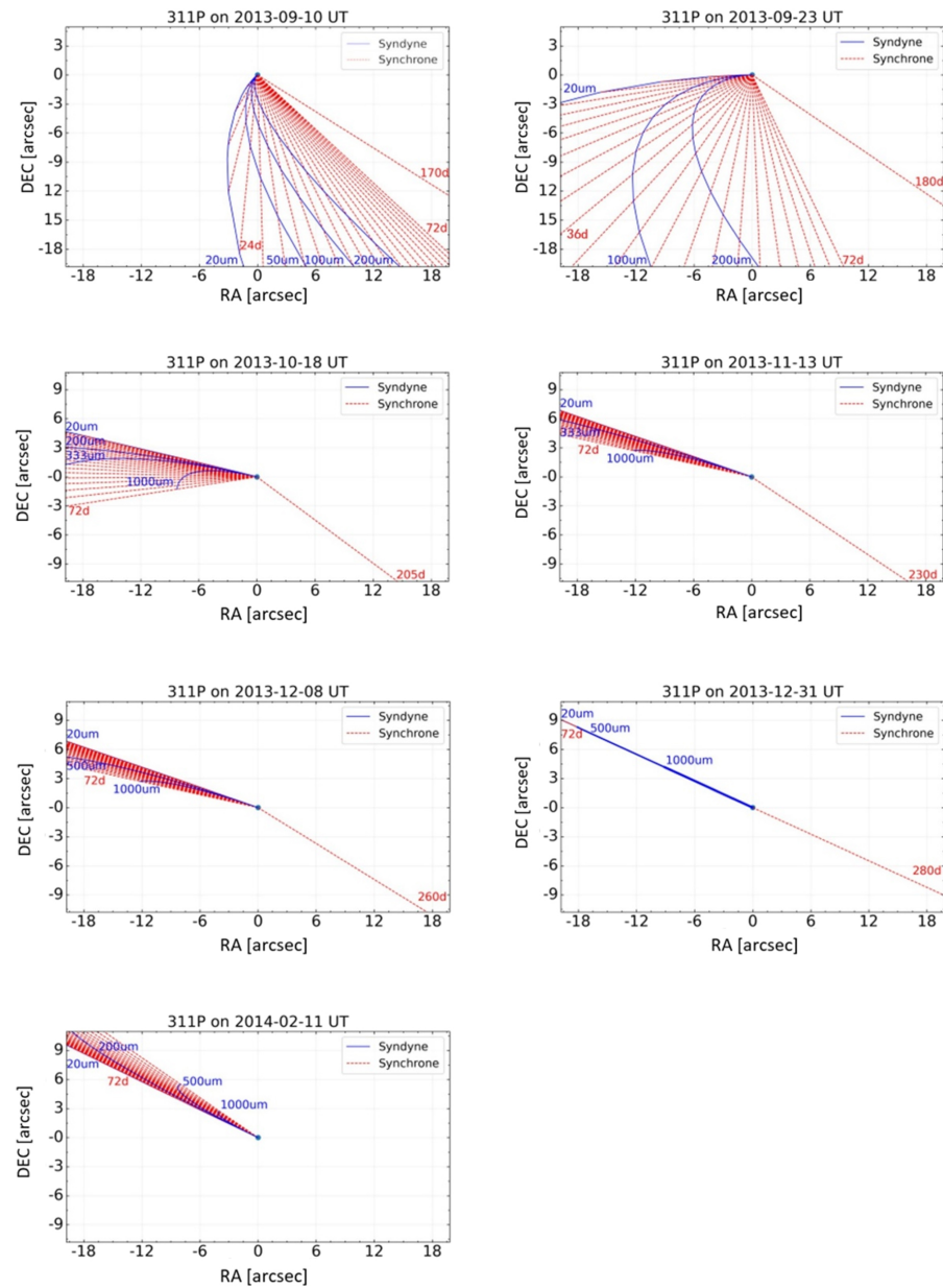
Figure 3. from Bin Liu et al 2023 Astron. J. 166 doi:10.3847/1538-3881/acf31c https://dx.doi.org/10.3847/1538-3881/acf31c © 2023. The Author(s). Published by the American Astronomical Society.
