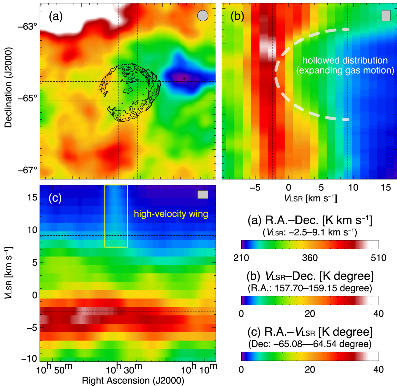
Figure 6. from Miroslav D. Filipovi et al 2023 Astron. J. 166 doi:10.3847/1538-3881/acf19c https://dx.doi.org/10.3847/1538-3881/acf19c © 2023. The Author(s). Published by the American Astronomical Society.
