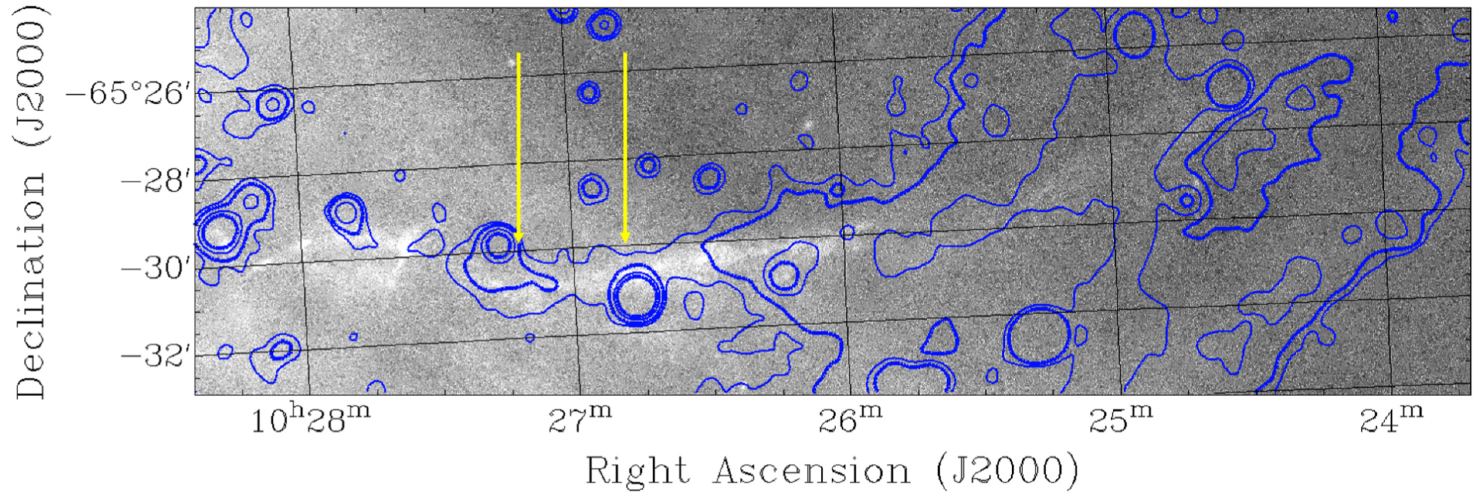
Figure 5. from Miroslav D. Filipovi et al 2023 Astron. J. 166 doi:10.3847/1538-3881/acf19c https://dx.doi.org/10.3847/1538-3881/acf19c © 2023. The Author(s). Published by the American Astronomical Society.
