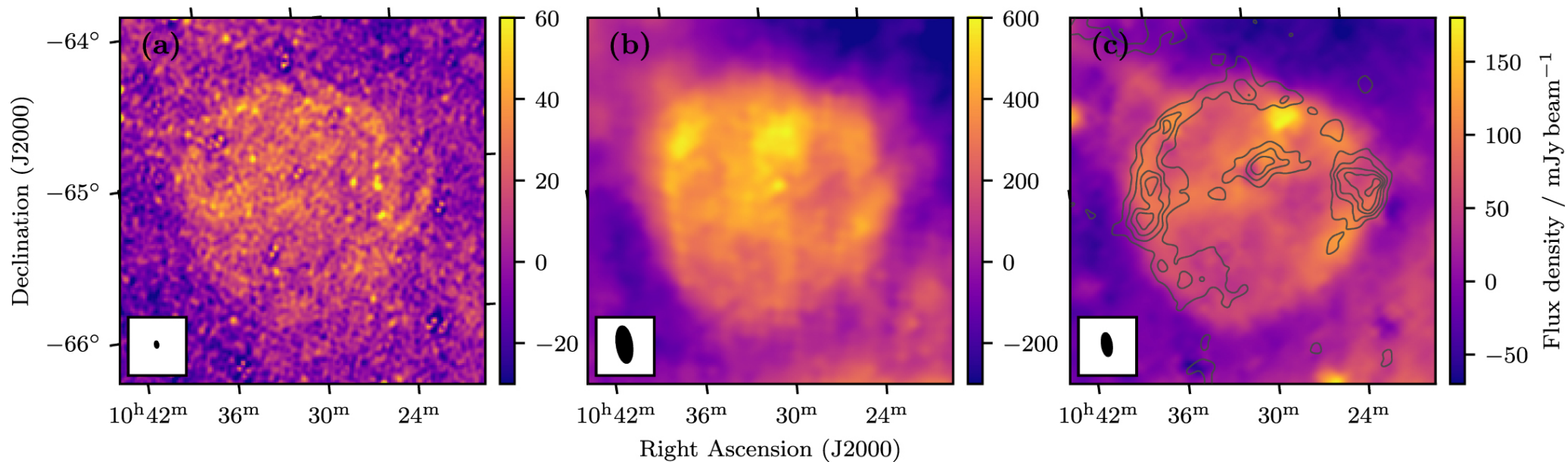
Figure 2. from Miroslav D. Filipovi et al 2023 Astron. J. 166 doi:10.3847/1538-3881/acf19c https://dx.doi.org/10.3847/1538-3881/acf19c © 2023. The Author(s). Published by the American Astronomical Society.
