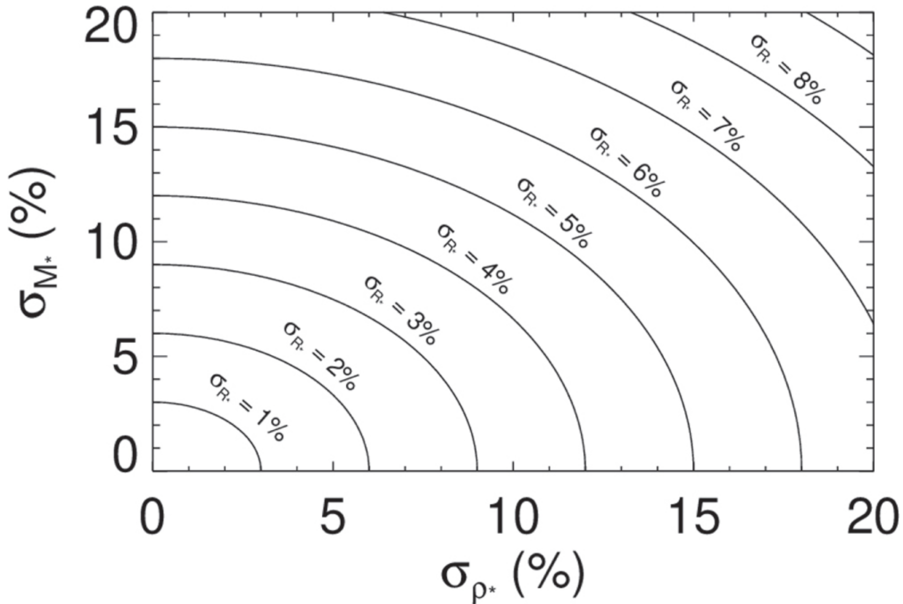
Figure 2. from Jason D. Eastman et al 2023 Astron. J. 166 doi:10.3847/1538-3881/aceda2 https://dx.doi.org/10.3847/1538-3881/aceda2 © 2023. The Author(s). Published by the American Astronomical Society.
