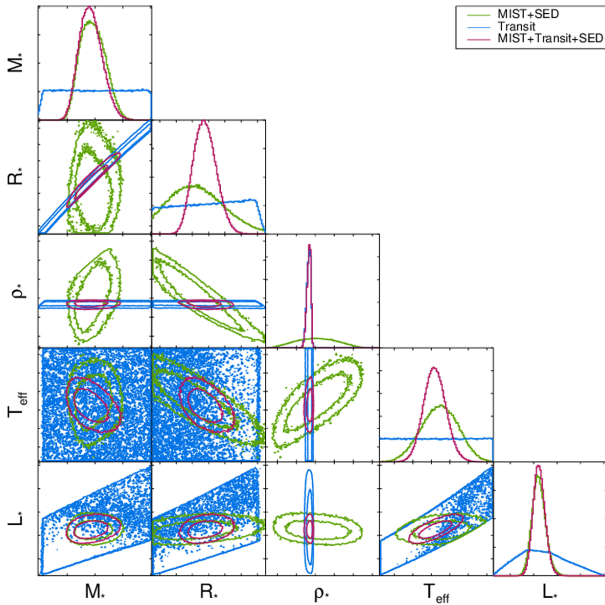
Figure 11. from Jason D. Eastman et al 2023 Astron. J. 166 doi:10.3847/1538-3881/aceda2 https://dx.doi.org/10.3847/1538-3881/aceda2 © 2023. The Author(s). Published by the American Astronomical Society.
