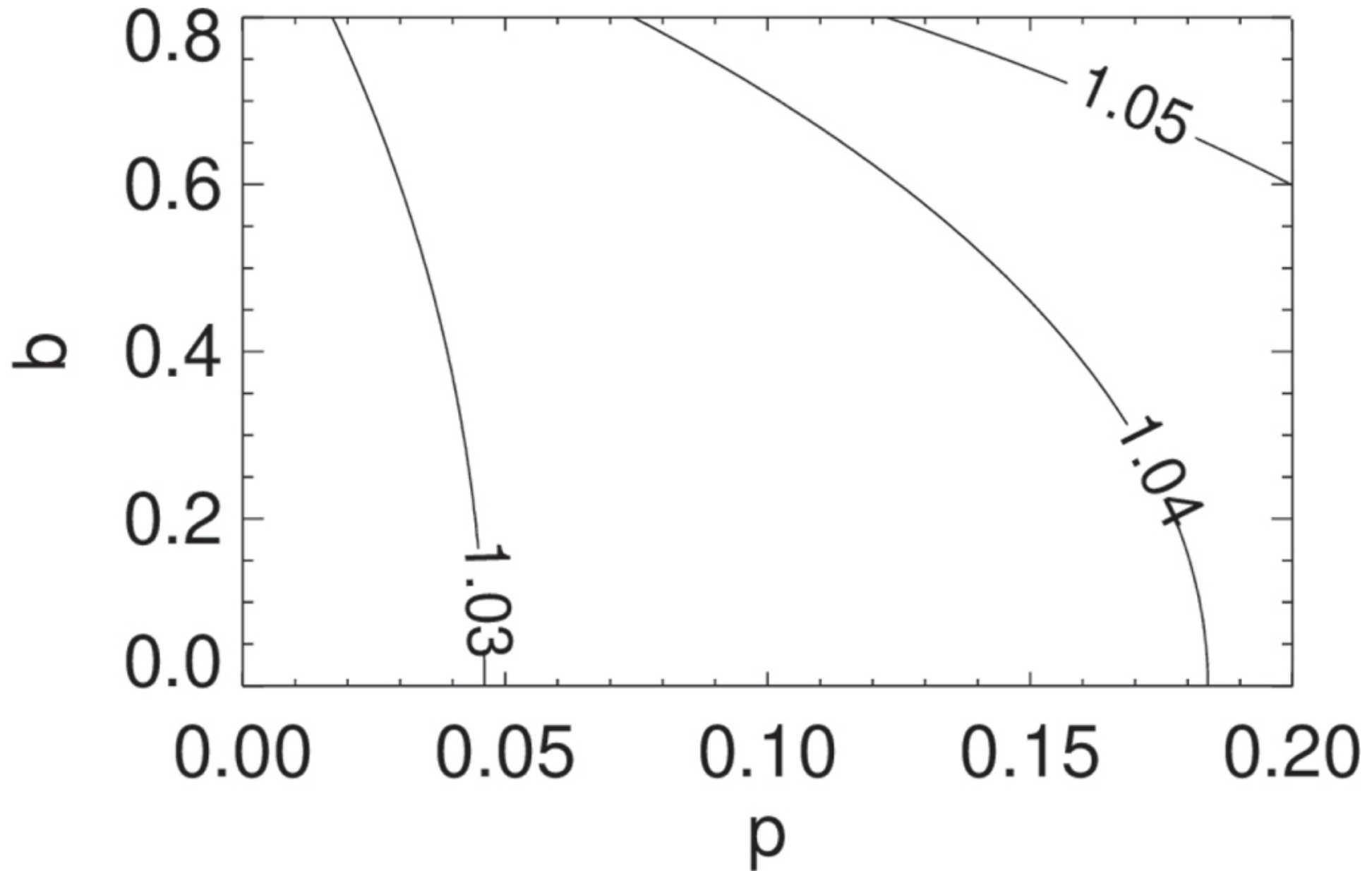
Figure 10. from Jason D. Eastman et al 2023 Astron. J. 166 doi:10.3847/1538-3881/aceda2 https://dx.doi.org/10.3847/1538-3881/aceda2 © 2023. The Author(s). Published by the American Astronomical Society.
