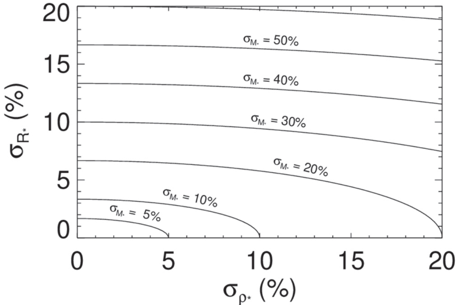
Figure 1. from Jason D. Eastman et al 2023 Astron. J. 166 doi:10.3847/1538-3881/aceda2 https://dx.doi.org/10.3847/1538-3881/aceda2 © 2023. The Author(s). Published by the American Astronomical Society.
