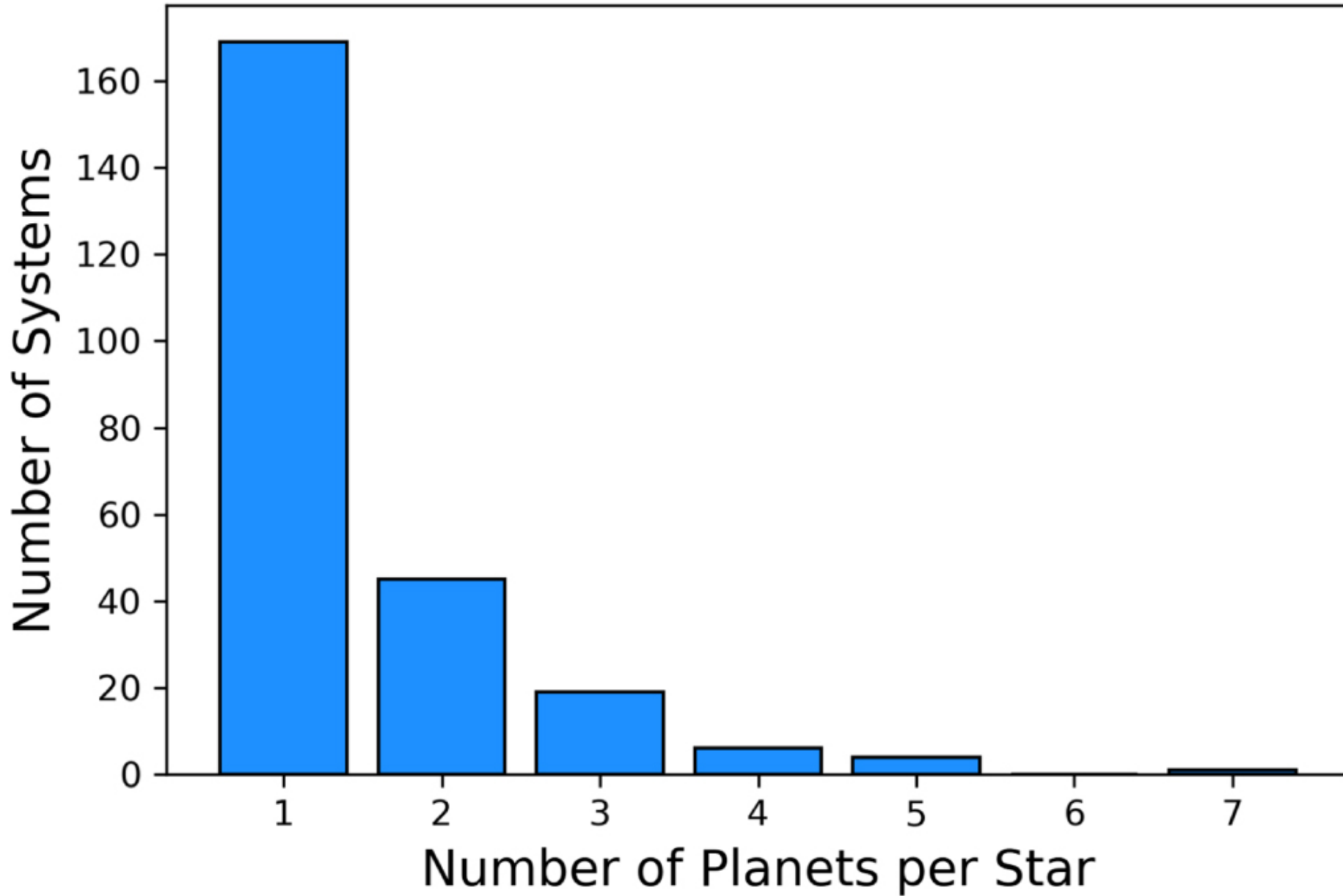
Figure 1. from Romy Rodríguez Martínez et al 2023 Astron. J. 166 doi:10.3847/1538-3881/aced9a https://dx.doi.org/10.3847/1538-3881/aced9a © 2023. The Author(s). Published by the American Astronomical Society.
