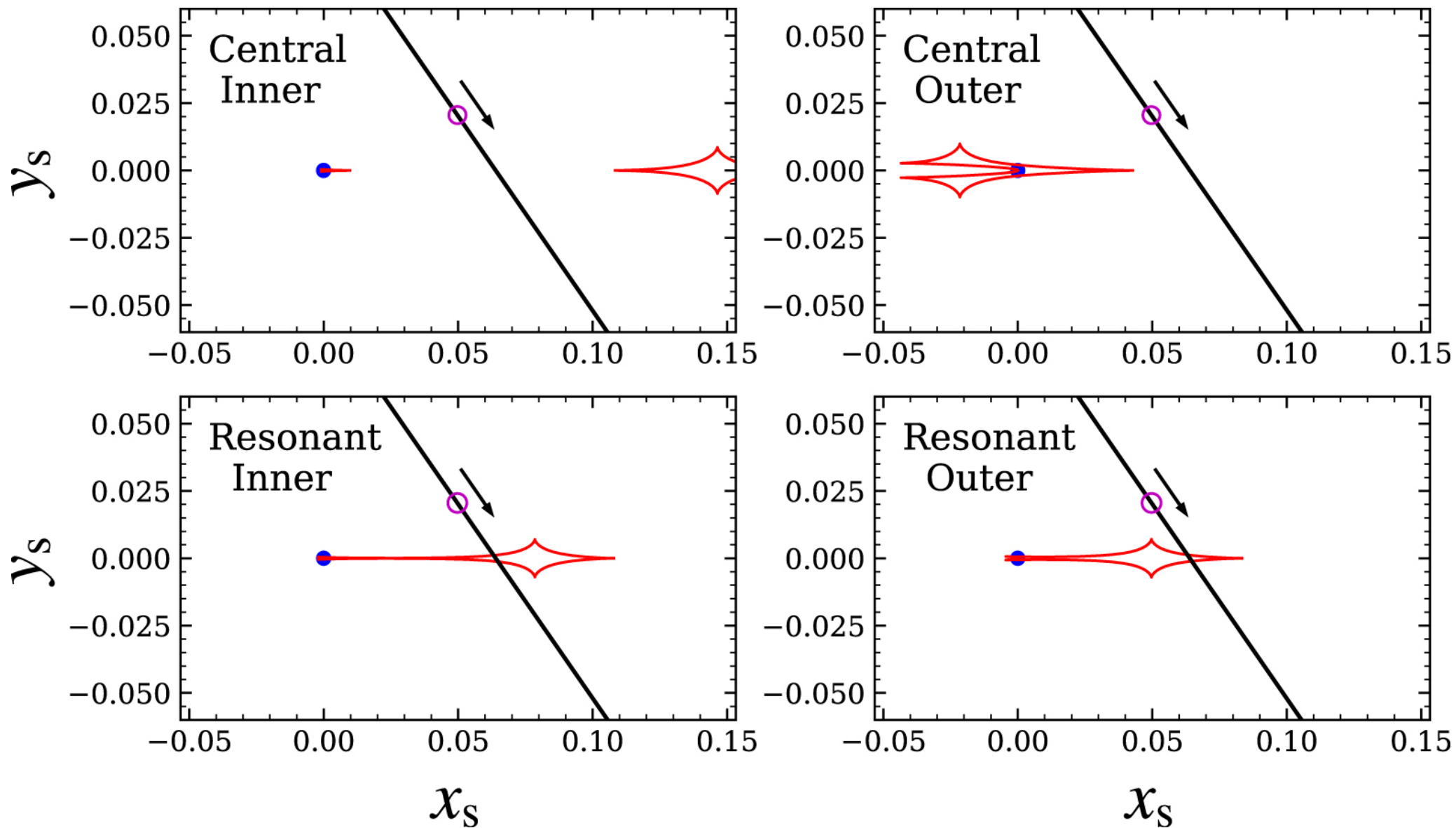
Figure 4. from Andrew Gould et al 2026 Astron. J. 166 doi:10.3847/1538-3881/aced3c https://dx.doi.org/10.3847/1538-3881/aced3c © 2023. The Author(s). Published by the American Astronomical Society.
