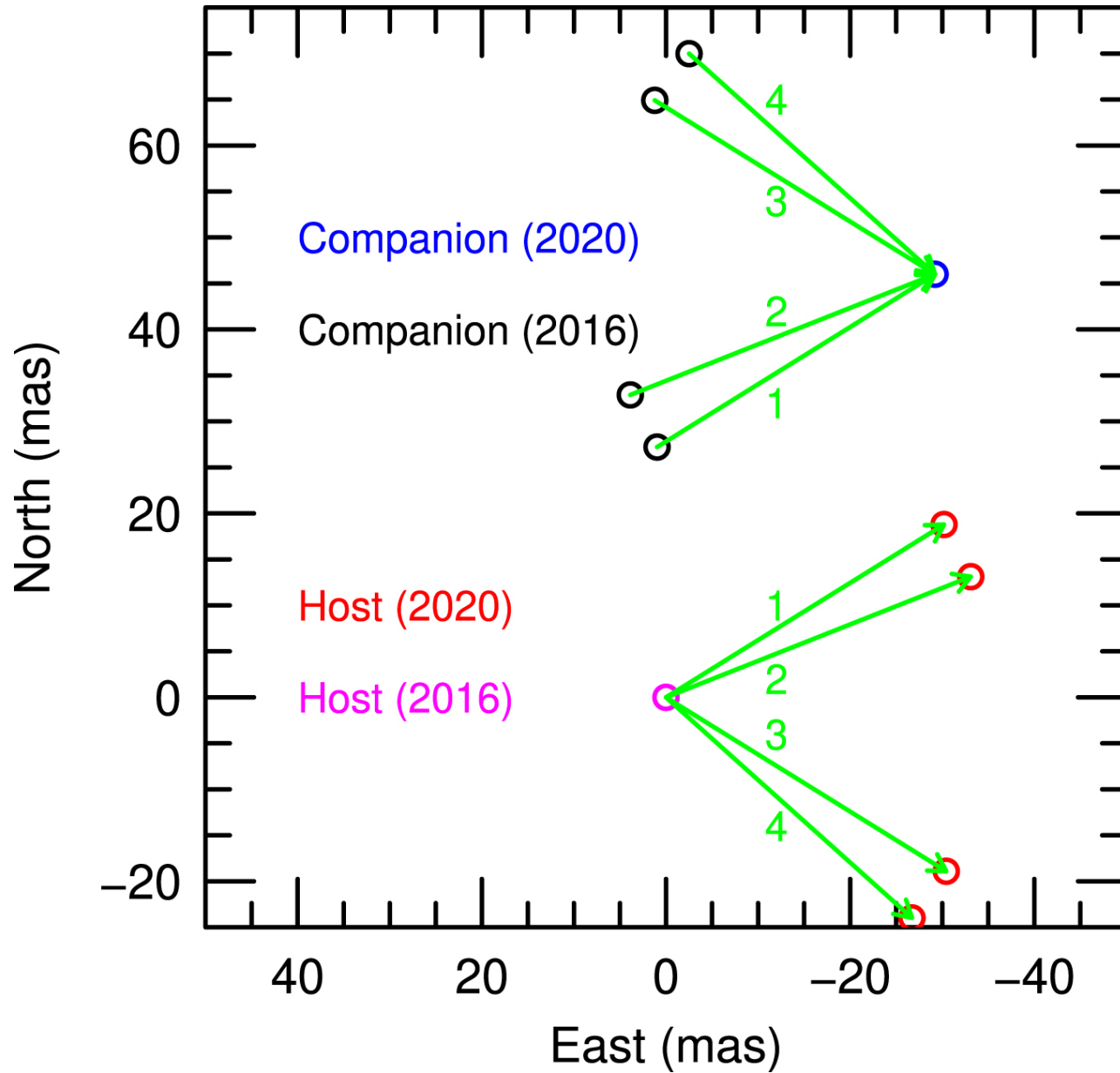
Figure 1. from Andrew Gould et al 2026 Astron. J. 166 doi:10.3847/1538-3881/aced3c https://dx.doi.org/10.3847/1538-3881/aced3c © 2023. The Author(s). Published by the American Astronomical Society.
