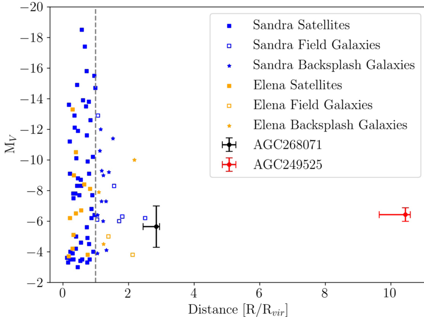
Figure 8. from Katherine L. Rhode et al 2023 Astron. J. 166 doi:10.3847/1538-3881/aceb5a https://dx.doi.org/10.3847/1538-3881/aceb5a © 2023. The Author(s). Published by the American Astronomical Society.
