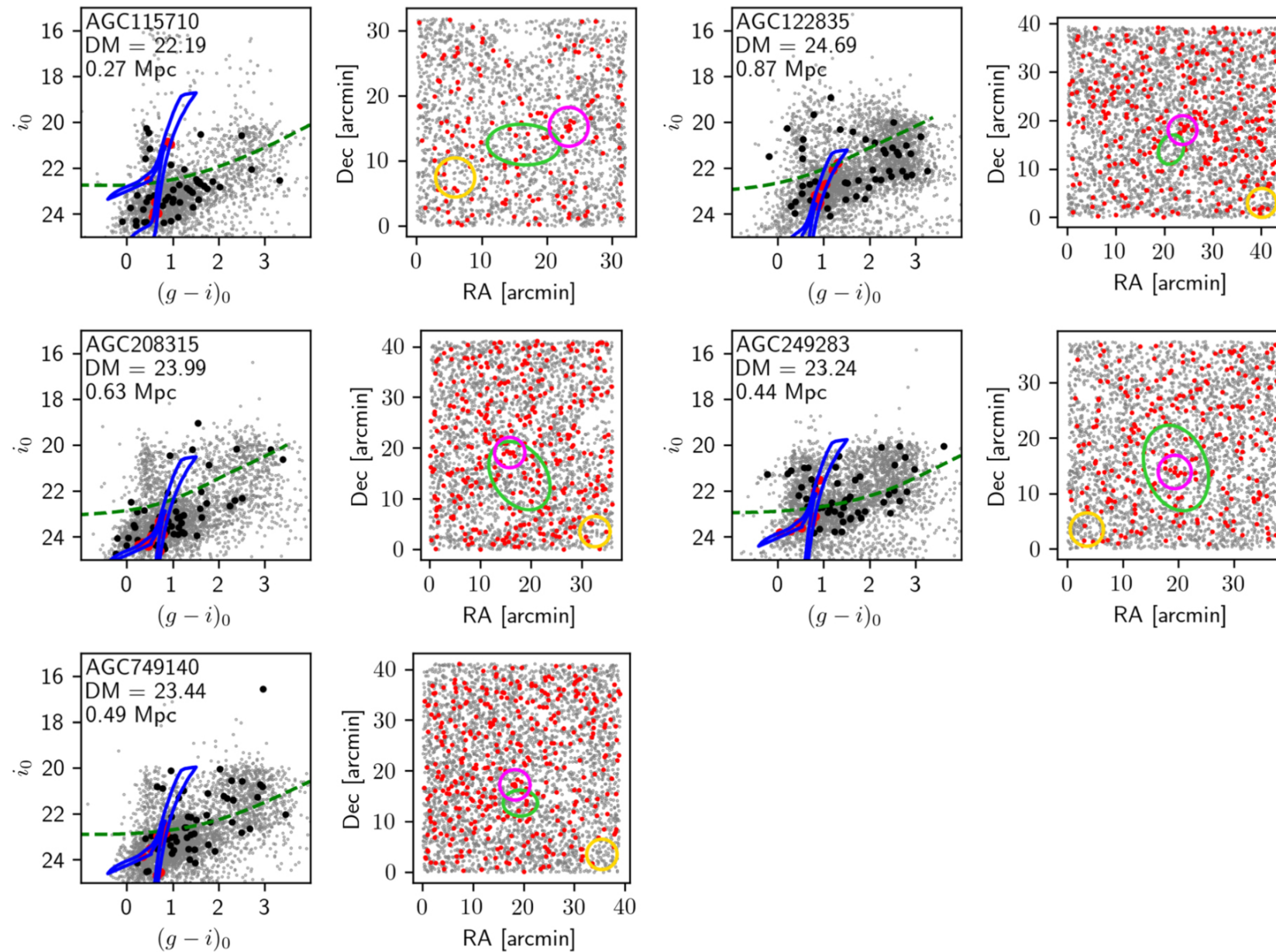
Figure 5. from Katherine L. Rhode et al 2023 Astron. J. 166 doi:10.3847/1538-3881/aceb5a https://dx.doi.org/10.3847/1538-3881/aceb5a © 2023. The Author(s). Published by the American Astronomical Society.
