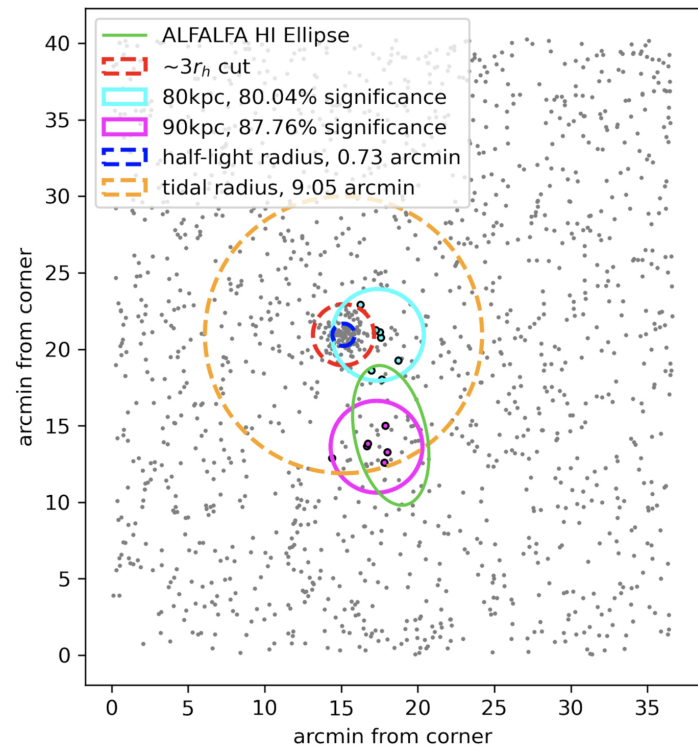
Figure 3. from Katherine L. Rhode et al 2023 Astron. J. 166 doi:10.3847/1538-3881/aceb5a https://dx.doi.org/10.3847/1538-3881/aceb5a © 2023. The Author(s). Published by the American Astronomical Society.
