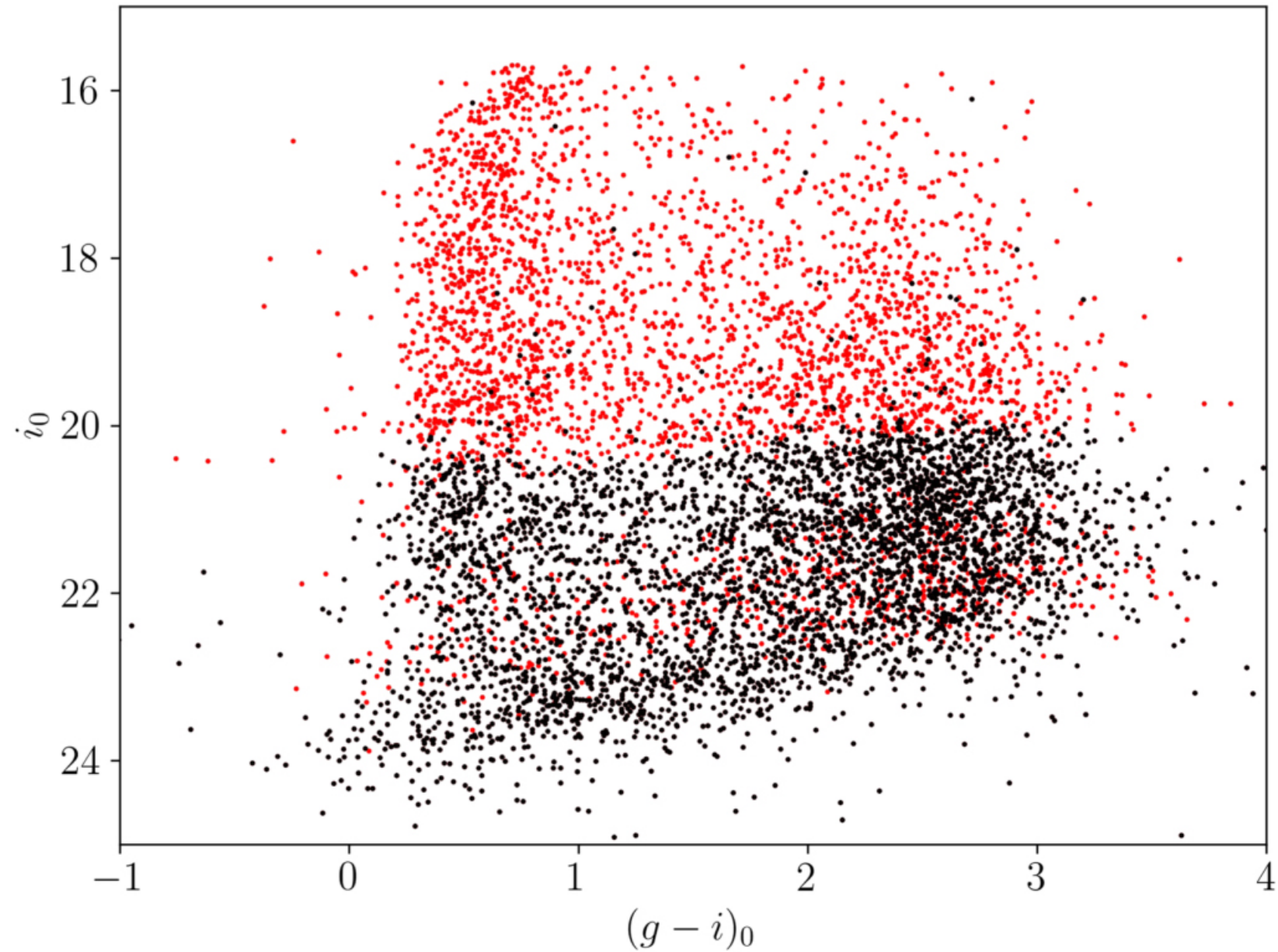
Figure 2. from Katherine L. Rhode et al 2023 Astron. J. 166 doi:10.3847/1538-3881/aceb5a https://dx.doi.org/10.3847/1538-3881/aceb5a © 2023. The Author(s). Published by the American Astronomical Society.
