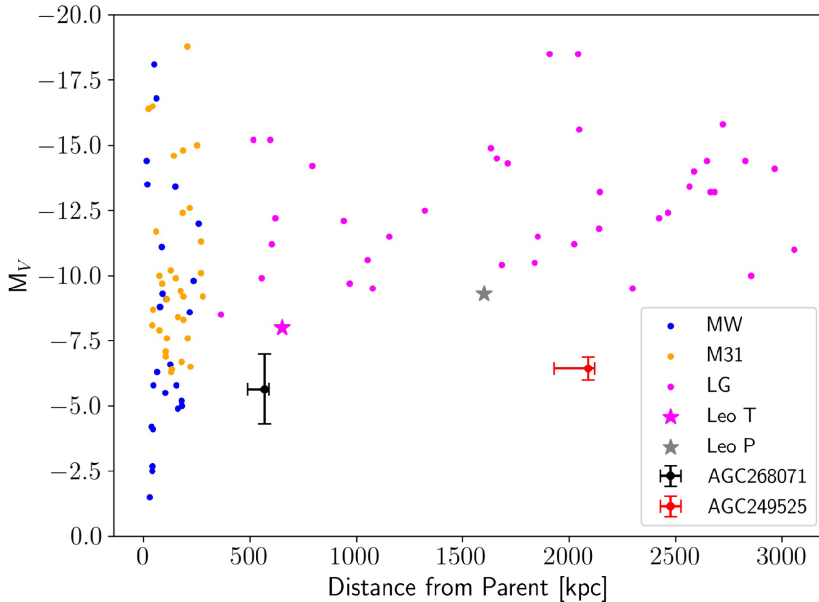
Figure 10. from Katherine L. Rhode et al 2023 Astron. J. 166 doi:10.3847/1538-3881/aceb5a https://dx.doi.org/10.3847/1538-3881/aceb5a © 2023. The Author(s). Published by the American Astronomical Society.
