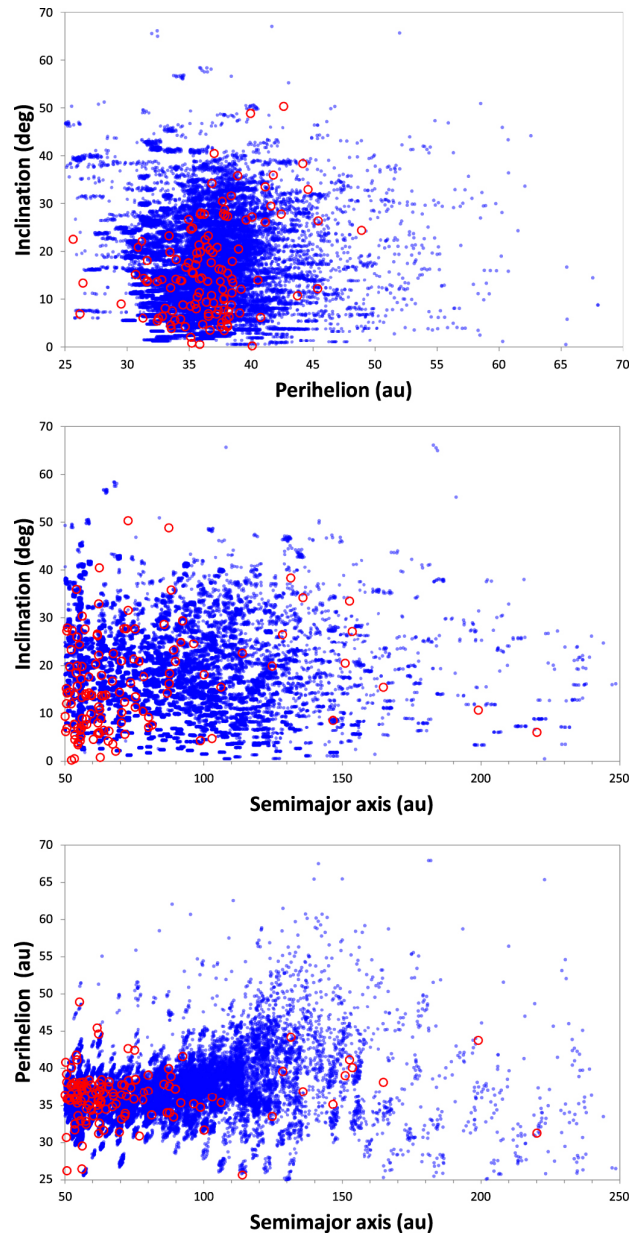
Figure 9. from Patryk Sofia Lykawka et al 2023 Astron. J. 166 doi:10.3847/1538-3881/aceaf0 https://dx.doi.org/10.3847/1538-3881/aceaf0 © 2023. The Author(s). Published by the American Astronomical Society.
