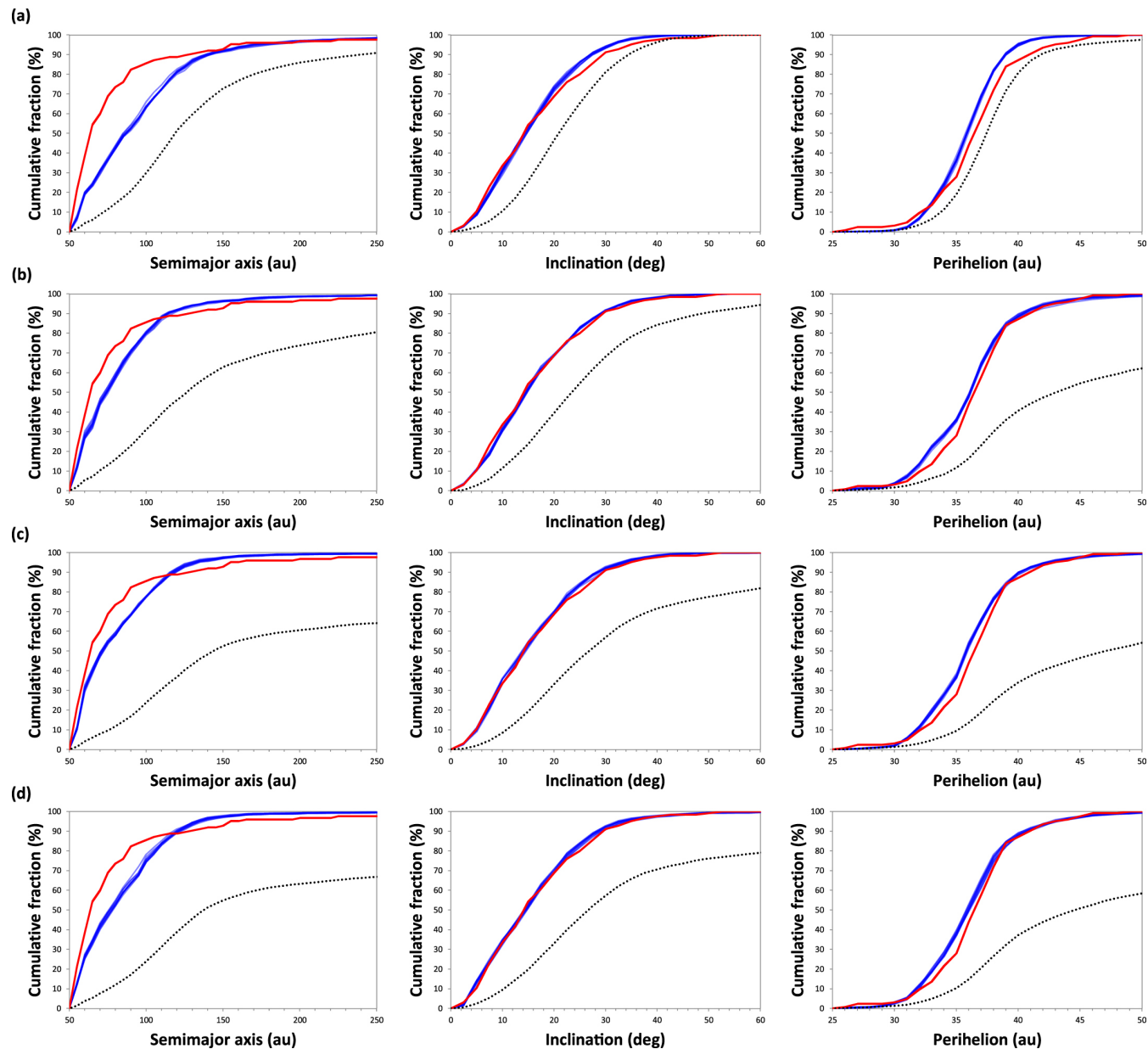
Figure 8. from Patryk Sofia Lykawka et al 2023 Astron. J. 166 doi:10.3847/1538-3881/aceaf0 https://dx.doi.org/10.3847/1538-3881/aceaf0 © 2023. The Author(s). Published by the American Astronomical Society.
