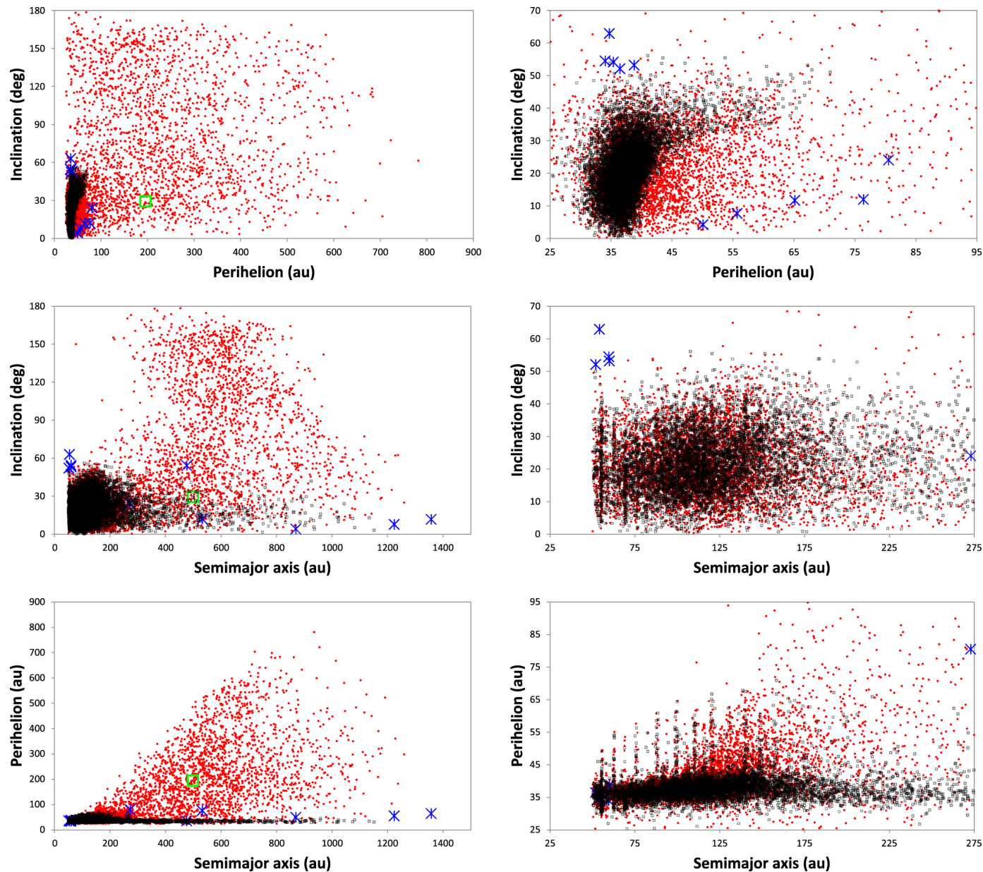
Figure 6. from Patryk Sofia Lykawka et al 2023 Astron. J. 166 doi:10.3847/1538-3881/aceaf0 https://dx.doi.org/10.3847/1538-3881/aceaf0 © 2023. The Author(s). Published by the American Astronomical Society.
